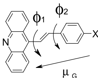
Scheme 3: Ground state structure of 1 . \phi_1 denotes the rotation of the acridine nucleus (considered to be planar) around the single bond to the central ethylene group; \phi_2 denotes the rotation of the para -substituted benzene ring around the single bond to the central ethylene group. \phi_1 : 55.5^\circ and \phi_2 : 169.2^\circ were found by X-Ray structure analysis for X = H.
