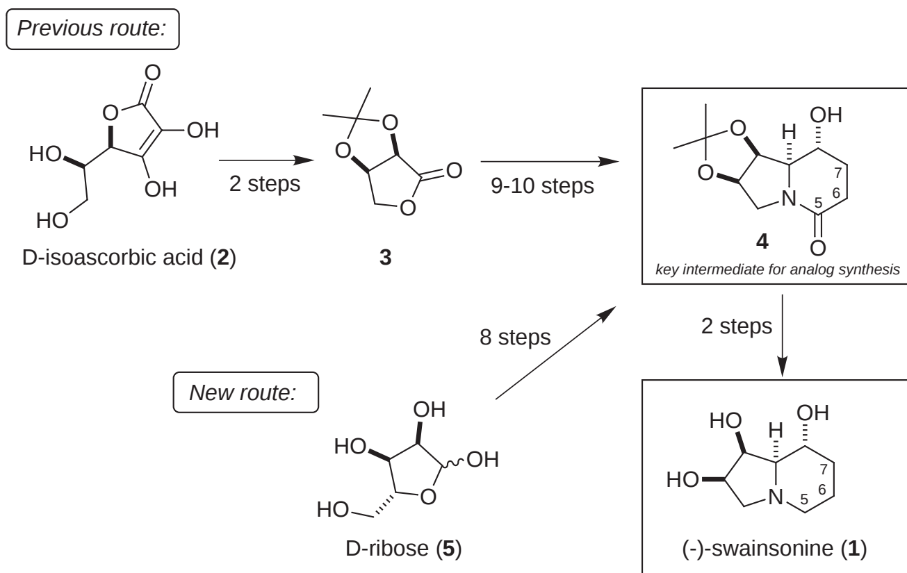
Scheme 1. Overview of (-)-swainsonine syntheses.
