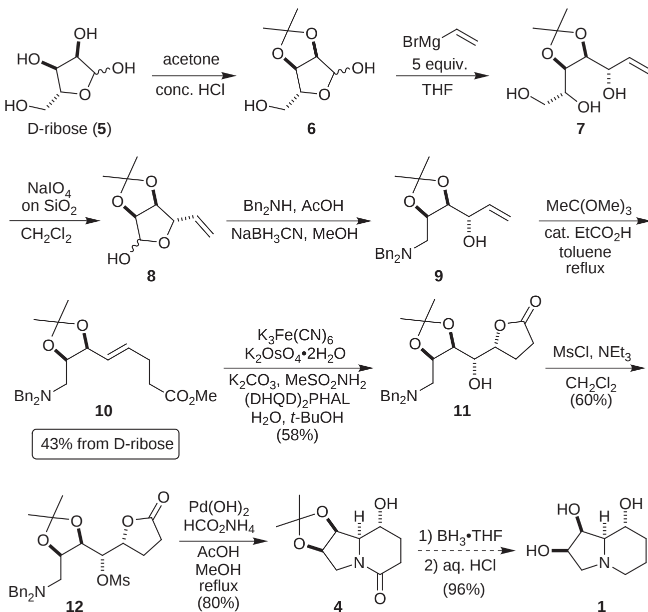
Scheme 2. Synthesis of swainsonine from D-ribose.
