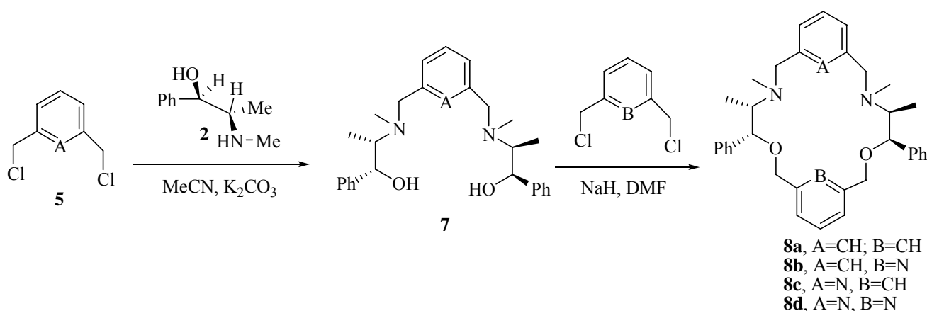
Scheme 3
