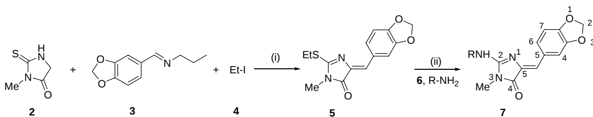
Scheme 1. Reagents and reaction conditions: (i) 2 1 equiv., 3 1 equiv., 4 1.5 equiv., K 2 CO 3 0.5 equiv., MeCN, 60°C, 14 h, 62%. (ii) 6 1-5 equiv., \mu\omega (Synthewave ® 402 reactor), 100-155°C, 20-100 min.
