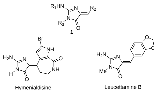
Figure 1. Structure of some marine alkaloids containing a ring of type 1
