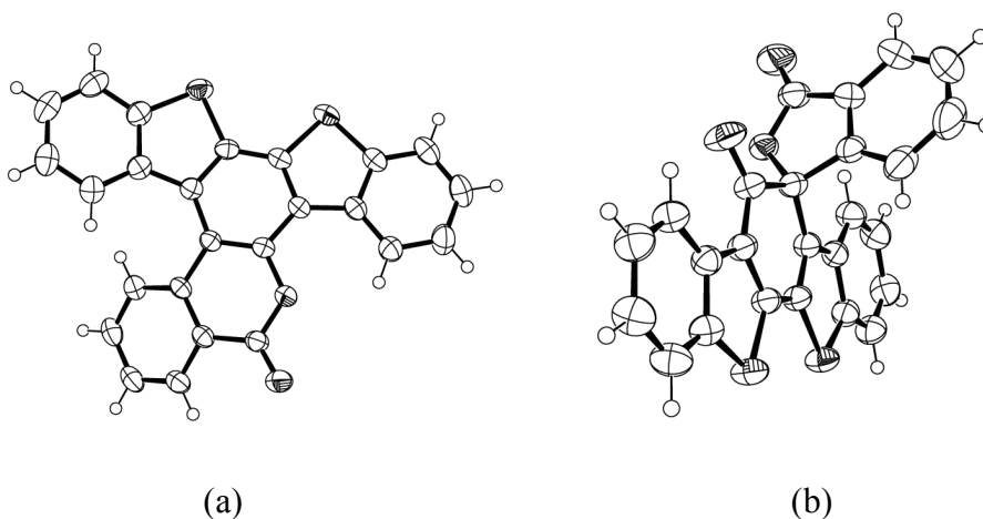
Figure 1 (a) ORTEP drawing of 6 . (b) ORTEP drawing of 7 .
