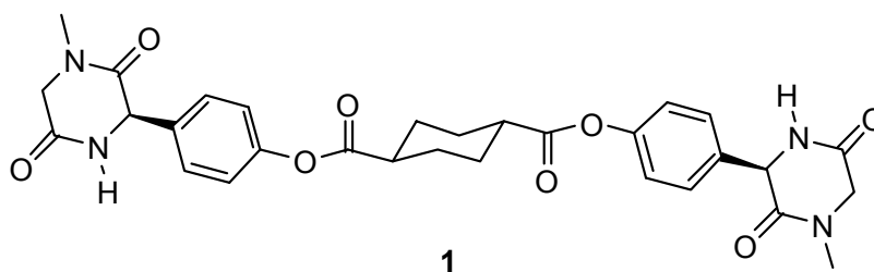
Figure 1. Structure of compound 1
