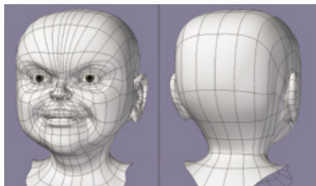
Figure 1—As mentioned, the face needs more geometry than the back of the head. Keeping areas like the back of the head simple will keep your mesh clean.
