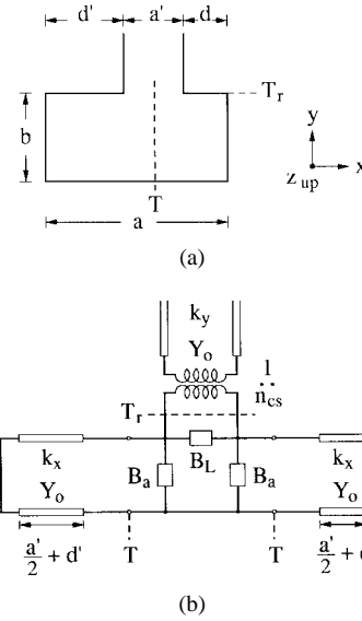
Fig. 2. (a) The cross section of the stub-loaded rectangular waveguide antenna. (b) Its transverse equivalent network, which utilizes the new E -plane tee junction equivalent network presented in [7].
