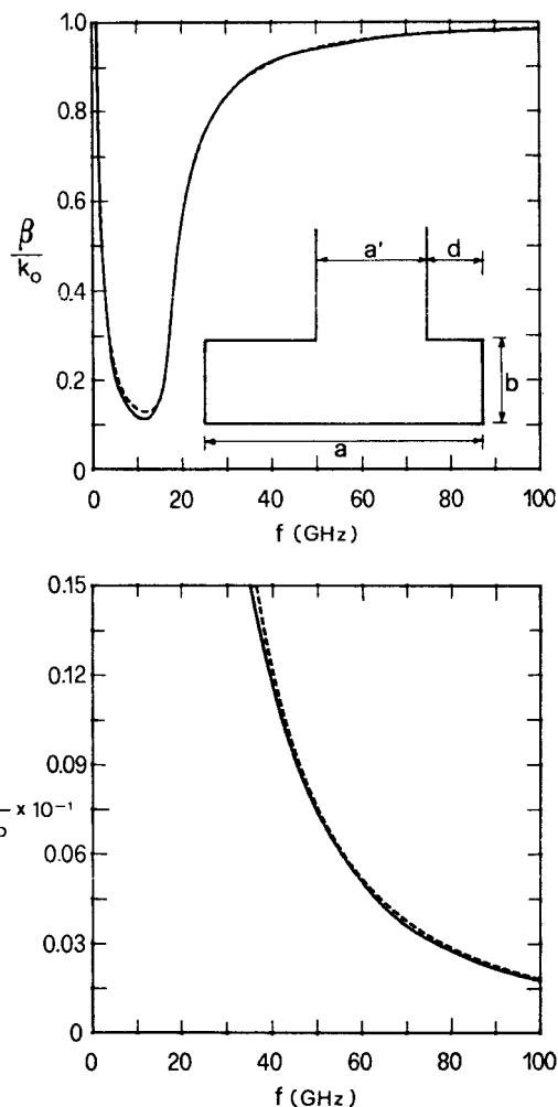
Fig. 4. Comparison of numerical results for \beta/k_0 and \alpha/k_0 versus frequency, over a very wide frequency range obtained via two completely different theoretical methods. The dashed and solid lines correspond, respectively, to the tee-junction network approach and the mode-matching procedure: a = 10.0 mm; b = 2.0 mm; a' = 4.0 mm; d = 2.0 mm.
