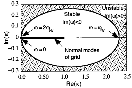
Fig. 1. Stability loop for a Debye material (water) with \epsilon_s = 81.0, \epsilon_\infty = 1.8 , and t_c = 9.4 \times 10^{-12} s, cell size of 37.5 \mu\text{m} , and Courant time step. Shaded areas are unstable. All normal modes are inside the loop, indicating that the region containing this material should be stable.
