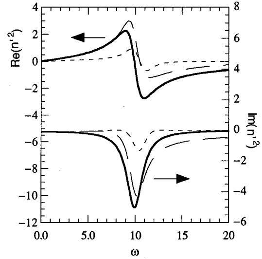
Fig. 5. Predicted numerical dispersion for Lorentz material with \epsilon_s = 1 , \epsilon_\infty = 0 , \omega_p = 10 , \delta_p = 1 , and \Delta_x = 0.0001 . Time steps are \delta_p \Delta_t = 0.0001 (heavy lines), \delta_p \Delta_t = 0.1 (long-dashed lines), and \delta_p \Delta_t = 0.3 (short-dashed lines).
