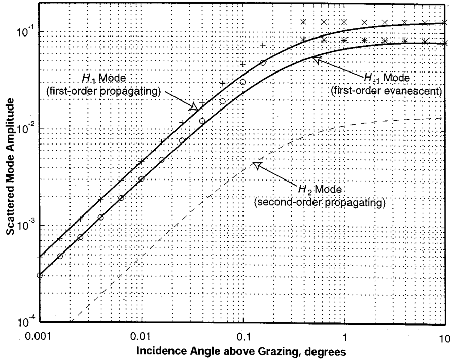
Fig. 1. Lowest order scattering amplitudes or modes. Curves are obtained from exact solutions for sinusoidal Neumann profile [9]. Points are first-order perturbation theory results; \times, * are "classic" perturbation theory predicting no grazing angle dependence, and +, o are grazing-limit perturbation theory derived herein.
