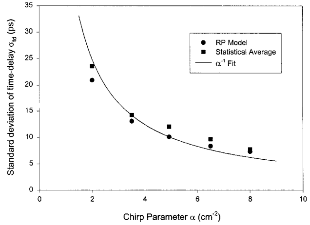
Fig. 13. Standard deviation for the time-delay \sigma_{td} at the center of the reflection band of the chirped grating versus the chirp parameter \alpha . The coherence length L_{coh} was kept constant to 100 cm. The solid line is the \alpha^{-1} fit.
