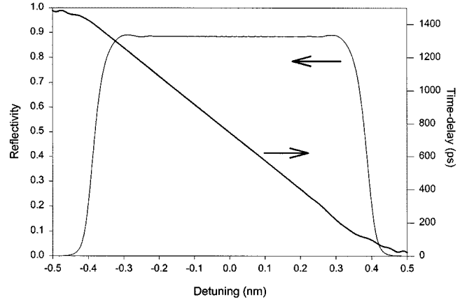
Fig. 10. Reflectivity and time-delay response for the chirped grating represented in Fig. 9.
