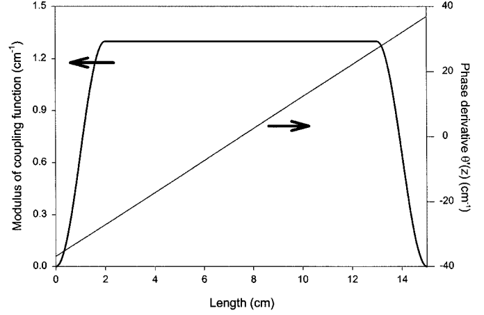
Fig. 9. Modulus and phase derivative of the deterministic coupling function q_o(z) for an apodized chirped grating.
