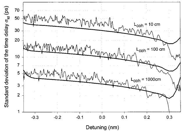
Fig. 11. Spectral evolution for the standard deviation of the time-delay \sigma_{td}(\beta) for different coherence lengths L_{\text{coh}} . The thick lines are the results predicted by the RP model, while the thin lines are statistical averages of 50 randomly generated chirped gratings.
