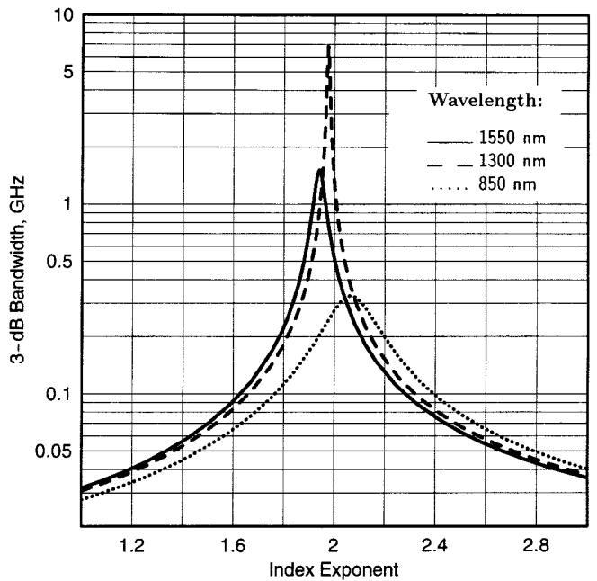
Fig. 3. 3-dBo baseband bandwidth of a 1014-m-long fiber as a function of refractive index exponent for wavelengths \lambda_0 = 850, 1300 , and 1550 \text{ nm} . All three curves are based on the results of analysis presented in [6].
