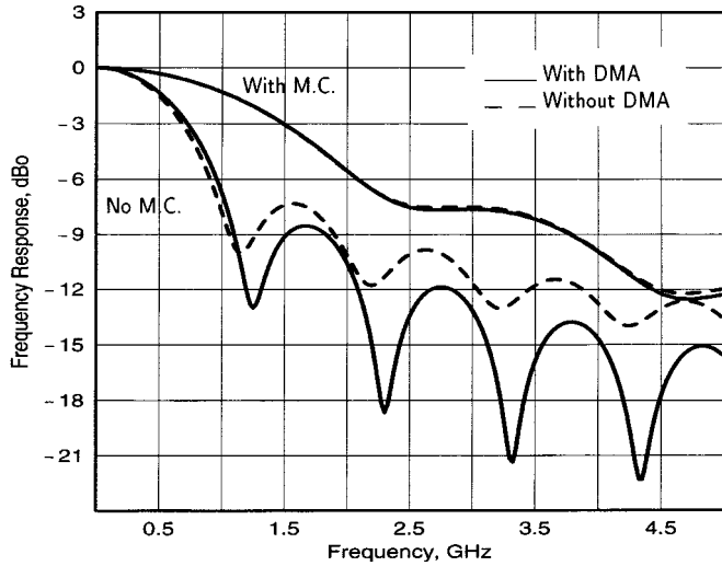
Fig. 7. Frequency responses of a 80/125 \mu\text{m} fiber showing the effect of differential mode attenuation (DMA) in presence and in absence of mode-coupling (M.C.): \lambda_0 = 1300 \text{ nm} , z = 2014 \text{ m} .
