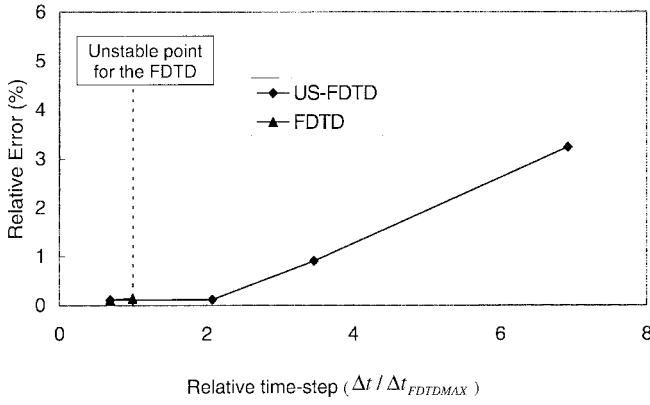
Fig. 2. Relative errors of the conventional FDTD and the proposed FDTD as the function of relative time step \Delta t / \Delta t_{FDTD\_MAX} . Dash line represents the unstable point of FDTD scheme.
