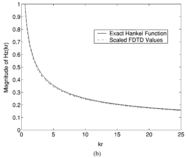
Fig. 1. |H_z(kr)| with scaled and unscaled FDTD values along the x axis for \lambda_0/5 grid resolution.
