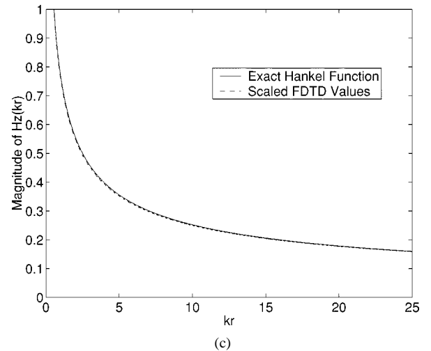
Fig. 2. Scatter diagram of |H_z(kr)| throughout the entire grid for three grid resolutions: (a) \lambda_0/5 ; (b) \lambda_0/10 ; (c) \lambda_0/20 .
