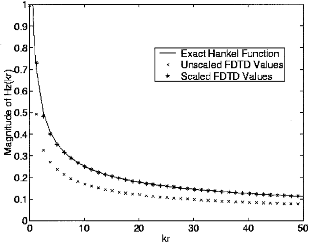
Fig. 1. |H_z(kr)| with scaled and unscaled FDTD values along the x axis for \lambda_0/5 grid resolution.
