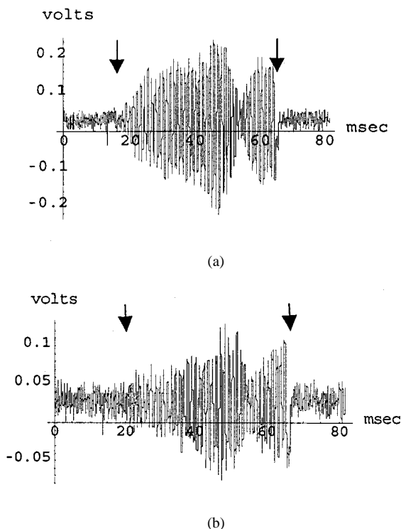
Fig. 2. Typical time domain waveforms for FM range measurement. Range = 1589 \text{ cm} \pm 0.6 \text{ cm} (a) Transponder on boresight. (b) Transponder at 75^\circ (E-plane rotation).
