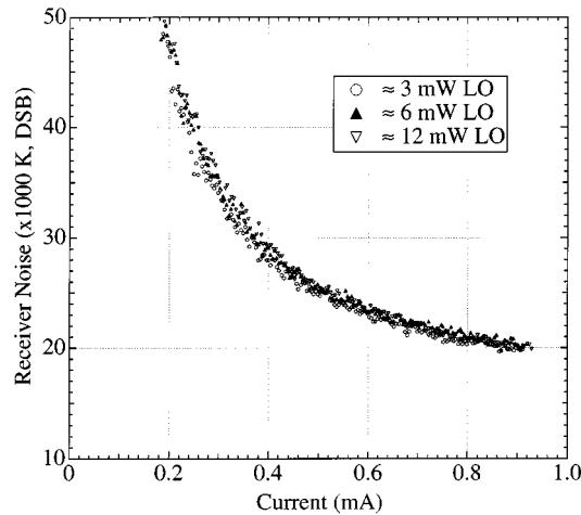
Fig. 9. Receiver noise versus current at an IF of 8.4 GHz, demonstrating the use of current bias to reduce sensitivity to LO fluctuations. A factor of \approx 4 in LO power results in virtually no input noise temperature change.
