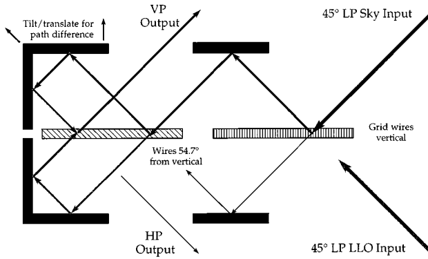
Fig. 2. Diplexer principle of operation. The right-hand-side grid splits the two input beams into two components for each beam. The heavy line follows the reflected half of the sky input (vertically polarized sky radiation). The left-hand-side grid splits this into two components, and interferometrically combines them after these two components are subjected to slightly different path lengths. The path length difference is adjusted such that the vertically polarized sky input at 12.8-GHz IF will pass through the “VP output” port. Sky inputs at 8.4- and 20.4-GHz IF will exhibit some cross-pol component due to compromises in the choice of path length. The LLO appears nearly horizontal at the HP port and nearly vertical at the VP port.
