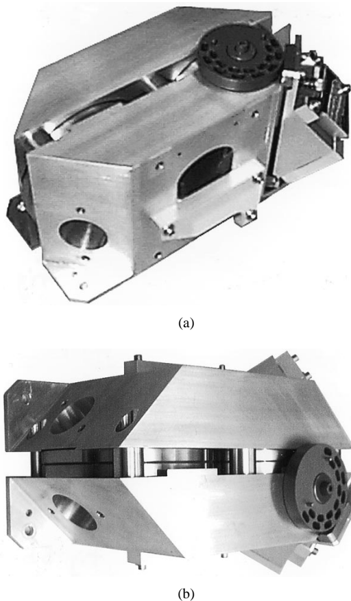
Fig. 5. Two views of the assembled 2.5-THz diplexer. (a) LO input port at bottom left-hand side, the vertical-polarization output in the center, and the adjuster wheel with tilting roof mirror at the top right. (b) Sky input at top left-hand side, a hint of the fixed roof mirror at top right-hand side, and the wire grid polarizer frames along the center.
