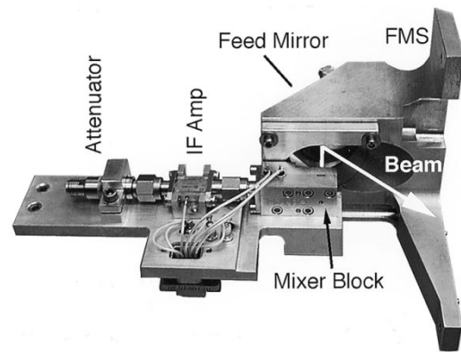
Fig. 6. Close-up of receiver front-end components. The chain includes an off-axis elliptical feed mirror, the mixer, a 7–22-GHz IF amplifier, and a clamped attenuator. Thermometry, amplifier power, and dc bias for the mixer passes through the connector at bottom. The feed mirror support (FMS) face to the right-hand-side bolts to a long edge of the hexagonal diplexer.
