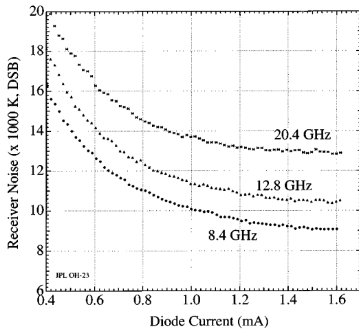
Fig. 11. Receiver noise versus current at intermediate frequencies of 8.4, 12.8, and 20.4 GHz. Filters with bandwidth of \approx 700 MHz were used to separate the intermediate frequencies. The LO power coupled to the mixer was approximately 7 mW.
