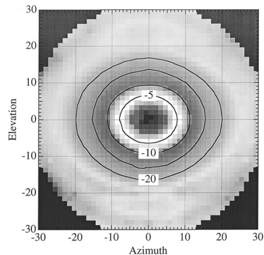
Fig. 7. JPL 2.5-THz Pickett–Potter horn beam pattern. Contours are in decibels.
