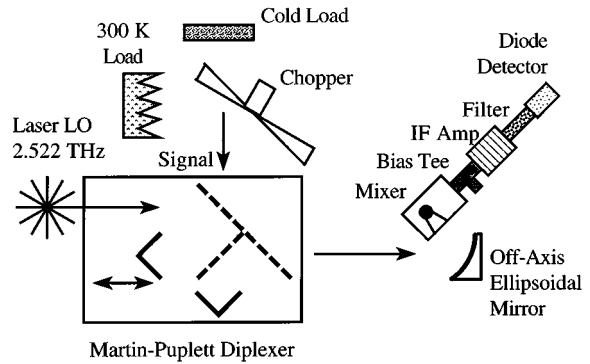
Fig. 10. Schematic of the 2.5-THz mixer test system. It is designed for sensitive measurement of high-noise devices, flexibility, and rapid computer-controlled measurements.
