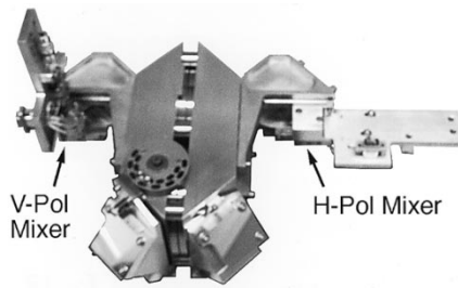
Fig. 13. Assembled receiver front end, in the configuration that was mounted on the electrodynamic shake table. Note the “vertical” mixer on the left-hand side, and the “horizontal” mixer on the right-hand side. The diplexer adjuster wheel is atop the roof mirror on the left-hand side.
