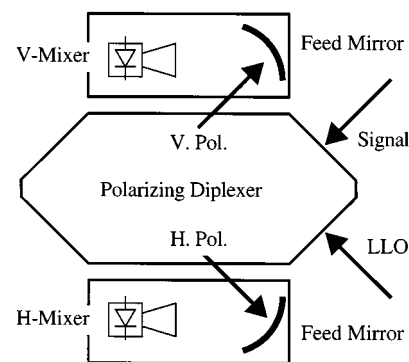
Fig. 1. Schematic diagram of the quasi-optical components in the 2.5-THz receiver front end.
