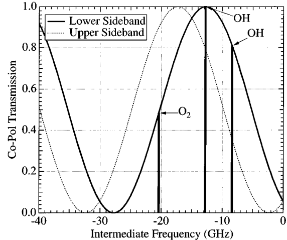
Fig. 3. Designed co-pol transmission of the sky signal through the 2.5-THz diplexer. The LLO beam will behave similarly, but with transmission curves identical to one minus the sky transmission. Note the opposite sideband rejection obtained for the OH channels by choice of path length difference (9.972 mm).
