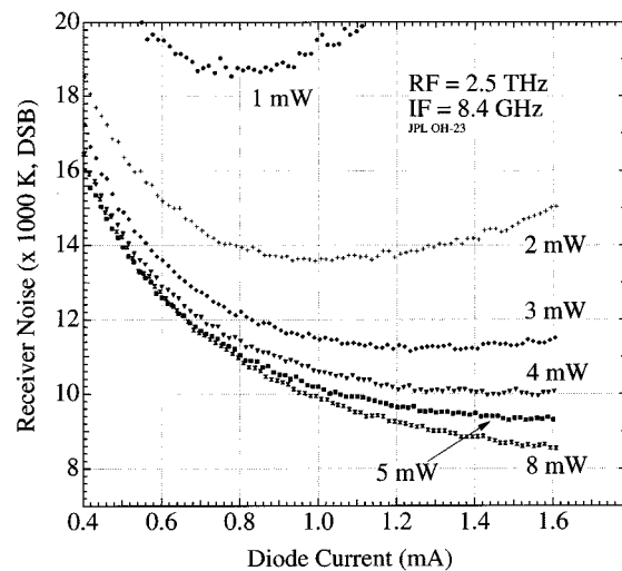
Fig. 12. Receiver noise versus current for various LO power levels. The IF is 8.4 GHz. Respectable performance is achieved with only 2 mW of coupled power.
