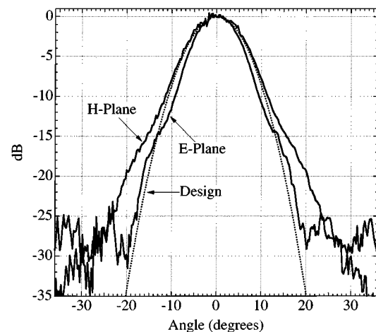
Fig. 8. JPL 2.5-THz Pickett–Potter horn beam pattern cuts in E - and H -planes, compared with the nominal design.
