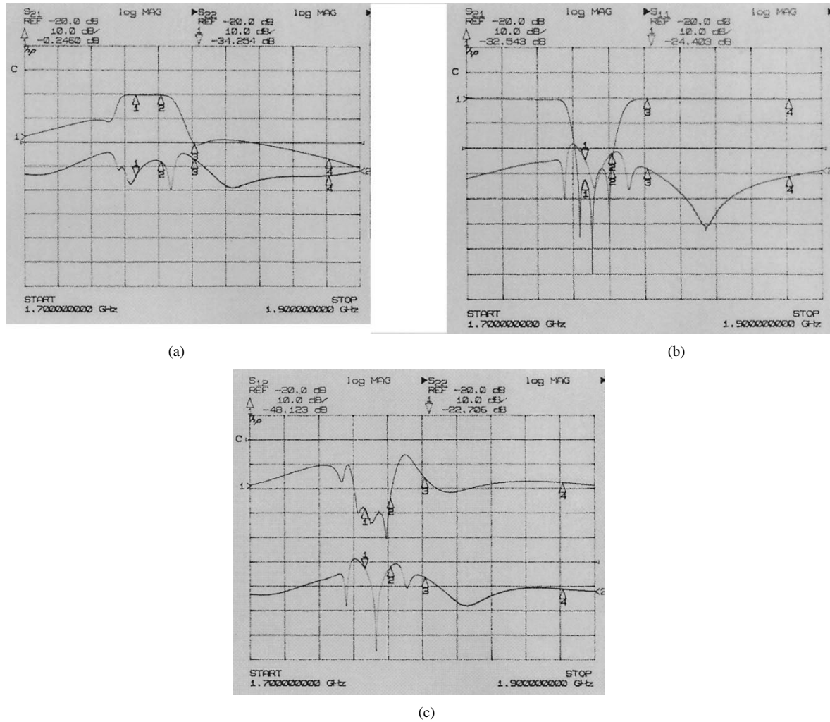
Fig. 10. Measured performance of the HTS duplexer in the test housing at T = 80 K. (a) Antenna-receiver. (b) Transmitter-antenna. (c) Transmitter-receiver.
