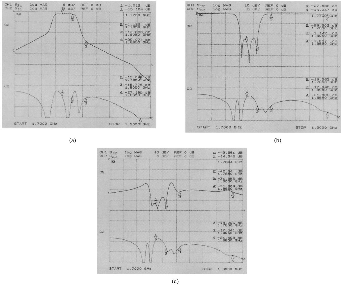
Fig. 12. Measured performance of an HTS duplexer in the encapsulated RF connector ring at a temperature of T = 55 K. (a) Antenna-receiver. (b) Transmitter-antenna. (c) Transmitter-receiver.
