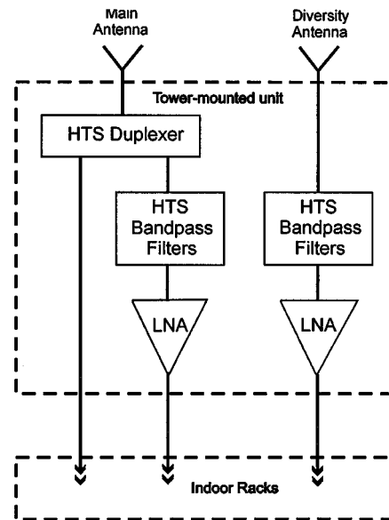
Fig. 1. Typical base-station sector using HTS subsystem.
