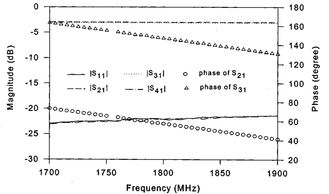
Fig. 5. Full-wave simulation of the HTS hybrid on an LAO substrate.
