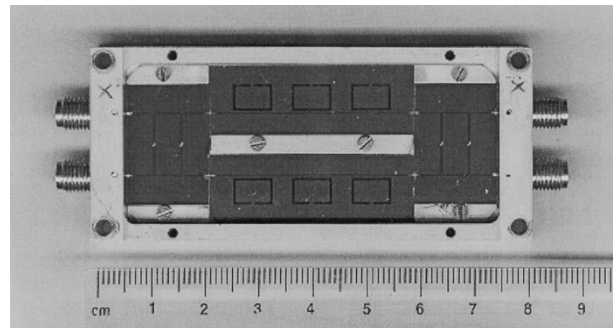
Fig. 8. Fabricated HTS duplexer in a test housing.
