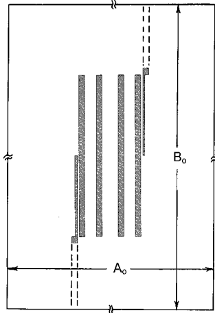
Fig. 1. Four-resonator-array test filter.
