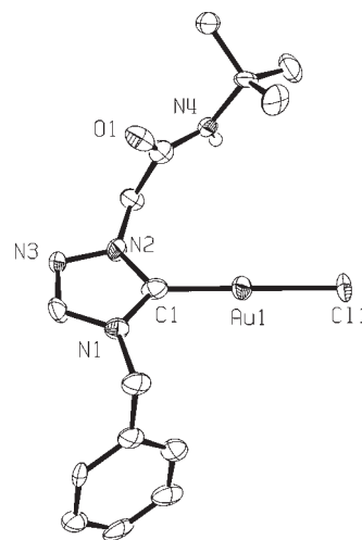
Figure 5. ORTEP drawing of 2c with thermal ellipsoids shown at the 50% probability level. Selected bond lengths (Å) and angles (deg): Au1–C1 1.950(10), Au1–Cl1 2.319(3), N1–C1 1.391(12), N2–C1 1.358(12), C1–Au1–Cl1 178.3(3), N1–C1–N2 101.1(8).
