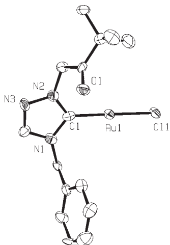
Figure 3. ORTEP drawing of 1c with thermal ellipsoids shown at the 50% probability level. Selected bond lengths (Å) and angles (deg): Au1–C1 1.972(12), Au1–Cl1 2.269(3), N1–C1 1.355(15), N2–C1 1.325(14), C1–Au1–Cl1 177.7(4), N1–C1–N2 104.0(10).
