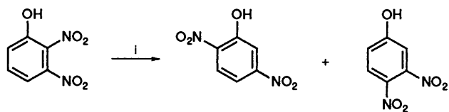
Scheme 1. Reagents and conditions: i, CF 3 SO 3 H, 100 °C.
