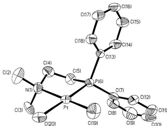
Figure 3. Molecular structure of 1 .
