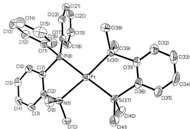
Figure 5. Molecular structure of 11 .
