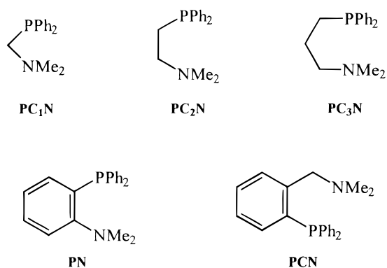
Figure 1. Employed P,N-chelating ligands.
