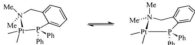
Figure 2. Conformational interconversion of the PCN ligand in complexes 4 , 9 , and 12 in solution.
