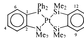
Figure 6. Atom labeling of the platinum complex 11 .
