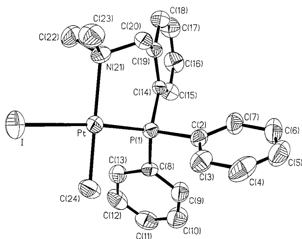
Figure 4. Molecular structure of 9 .
