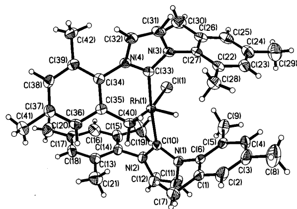
Figure 1. ORTEP of Rh(IMes)(H)(IMes)Cl ( 2 ) with ellipsoids drawn at 50% probability. Selected bond distances and angles: Rh(1)-C(33), 2.0242(17); Rh(1)-C(10), 2.0480(17); Rh(1)-C(40), 2.0793(18); Rh(1)-Cl(1), 2.4363(5); Rh(1)-H(1), 1.455(17); C(33)-Rh(1)-C(10), 172.33(7); C(33)-Rh(1)-C(40), 81.21(7); C(10)-Rh(1)-C(40), 95.66(7); C(33)-Rh(1)-Cl(1), 93.05(5); C(10)-Rh(1)-Cl(1), 91.13(5); C(40)-Rh(1)-Cl(1), 169.07(5); C(33)-Rh(1)-H(1), 87.4(7); C(10)-Rh(1)-H(1), 85.3(7); C(40)-Rh(1)-H(1), 83.5(7); Cl(1)-Rh(1)-H(1), 105.6(7).
