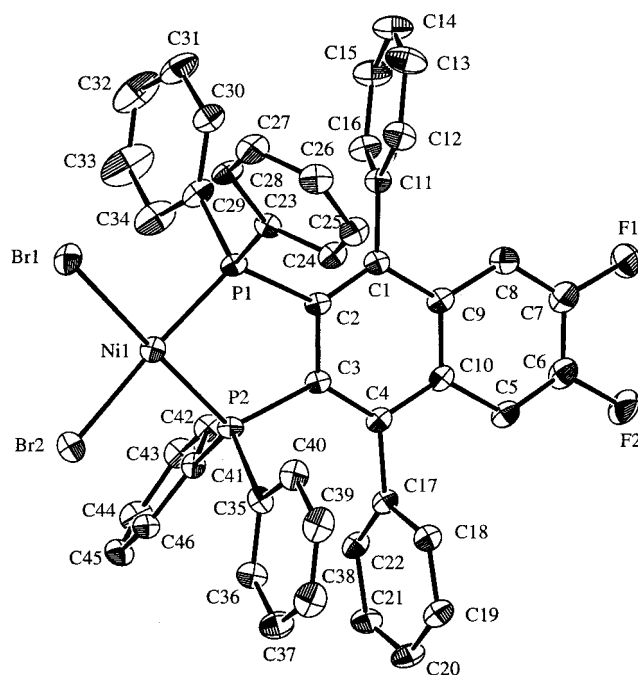
Figure 1. Molecular structure of 11b with selected atom labeling. Thermal ellipsoids show 30% probability levels; hydrogen atoms have been omitted for clarity.
