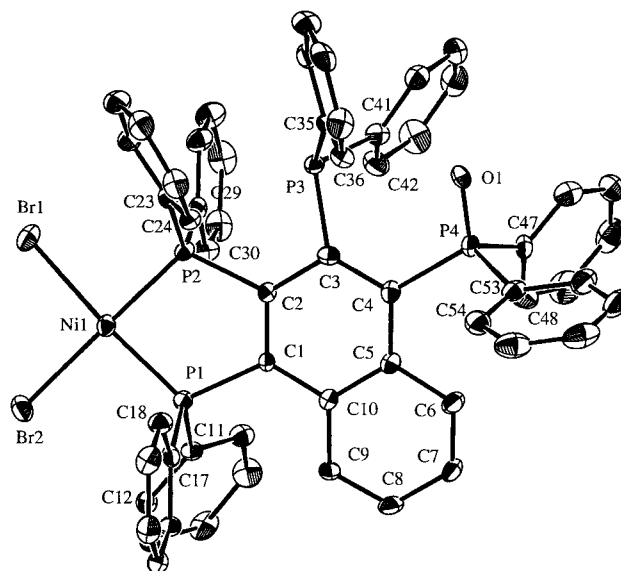
Figure 2. Molecular structure of 18 with selected atom labeling. Thermal ellipsoids show 30% probability levels; hydrogen atoms have been omitted for clarity.
