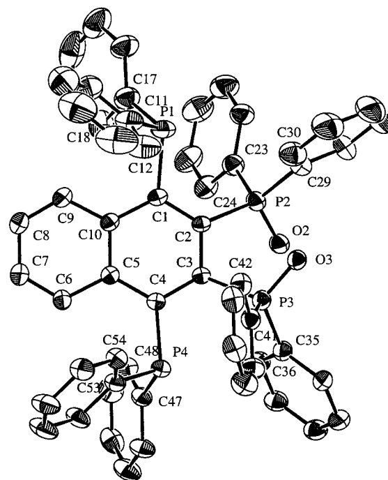
Figure 3. Molecular structure of 20 with selected atom labeling. Thermal ellipsoids show 30% probability levels; hydrogen atoms have been omitted for clarity.
