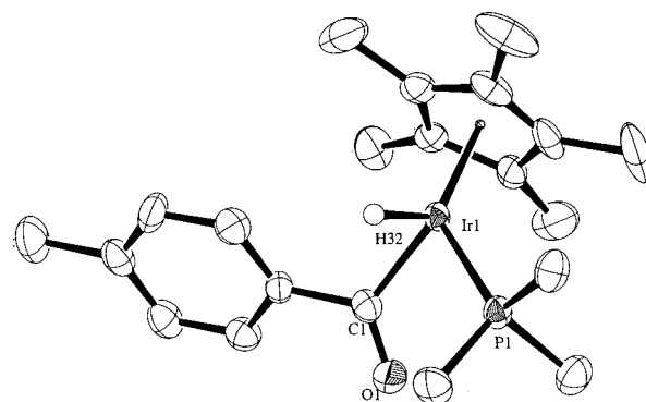
Figure 1. ORTEP diagram of Cp*(PMe 3 )Ir(C(O) p -CH 3 C 6 H 4 )(H) ( 3b ). Thermal ellipsoids are shown at 50% probability levels. Hydrogen atoms (except H32) are omitted for clarity.
