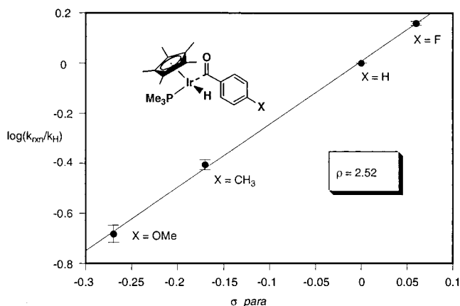
Figure 5. Hammett correlation for the reaction of 1a with para-substituted benzoyl chlorides in the presence of 7 .
