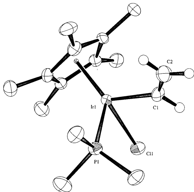
Figure 7. ORTEP diagram of \text{Cp}^*(\text{PMe}_3)\text{Ir}(\text{CH}=\text{CH}_2)\text{Cl} . Thermal ellipsoids are shown at 50% probability levels. Hydrogen atoms (except on the vinyl moiety) are omitted for clarity.
