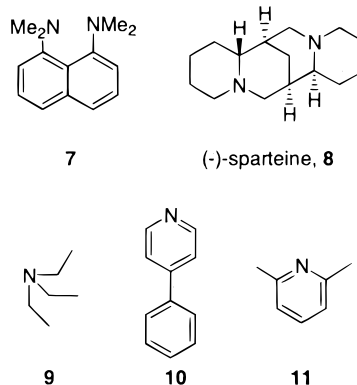
Figure 6. Amines used in the kinetic study.
