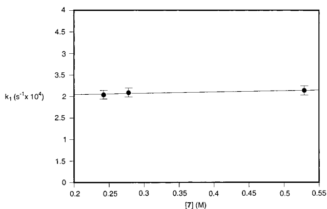
Figure 4. Rate dependence on [7] measured using flooding conditions for the reaction with 1a and 2a .
