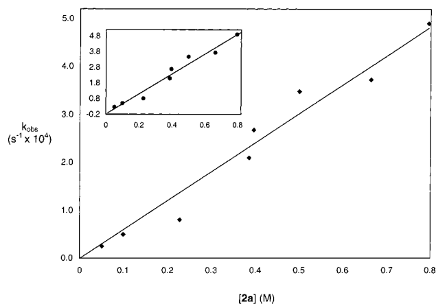
Figure 3. Rate dependence on [2a] using flooding conditions for the reaction with 1a and 7 ( R^2 = 0.96 ) with the intercept set at zero. Inset: Same rate dependence plot with intercept not set at zero ( R^2 = 0.97 ).
