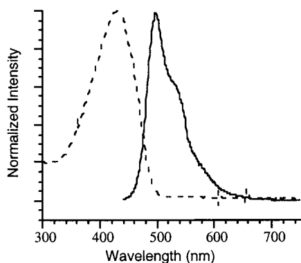
Figure 2. Absorption (---) and emission (—) spectra of 7b ( M_n = 4700 ).
