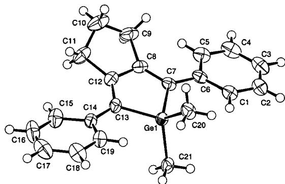
Figure 1. X-ray crystallographic structure of model compound 6 .
