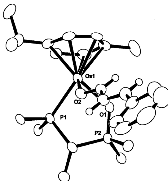
Figure 4. ORTEP diagram of 4a showing 50% probability ellipsoids. The phenyl groups of the phosphines are omitted for clarity. The compound is racemic, and the ( R Os , S C )-enantiomer is shown.
