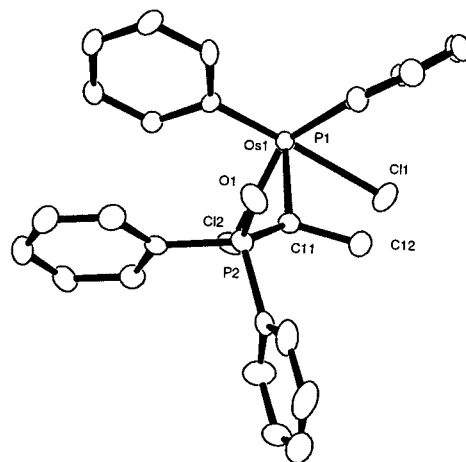
Figure 5. ORTEP diagram of 1 showing 50% probability ellipsoids illustrating the conformation of the phenyl rings. The compound is racemic, and the ( S D )-enantiomer is shown. The cymene group has been omitted for clarity.
