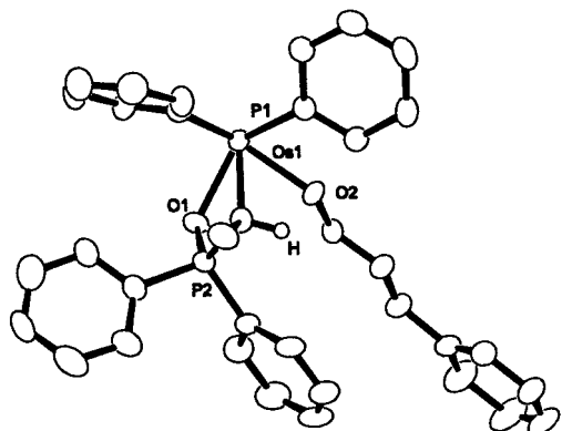
Figure 7. ORTEP view of 4a showing 50% probability ellipsoids illustrating the conformation of the phenyl rings. The compound is racemic, and the ( S C )-enantiomer is shown. The cymene group has been omitted for clarity.
