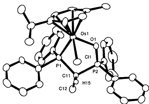
Figure 3. ORTEP diagram of cation 2a showing 50% probability ellipsoids. The compound is racemic, and the ( R Os , S C )-enantiomer is shown.
