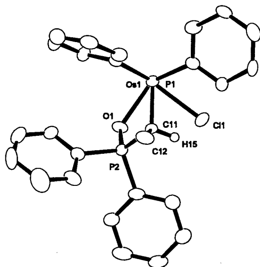
Figure 6. ORTEP view of 2a showing 50% probability ellipsoids illustrating the conformation of the phenyl rings. The compound is racemic, and the ( S C )-enantiomer is shown. The cymene group has been omitted for clarity.
