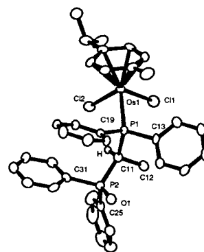
Figure 1. ORTEP diagram of 1 showing 50% probability ellipsoids. The compound is racemic, and the ( S C )-enantiomer is shown. Note that the chirality descriptor at carbon changes upon binding of the ligand; hence the ( R C )-BPMO free ligand becomes ( S C ) when the phosphine binds to a transition metal.
