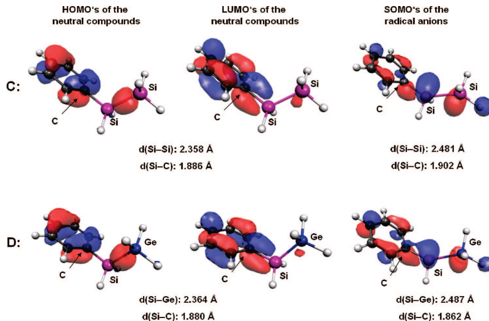
Figure 4. HOMOs (left) and LUMOs (middle) of the two neutral model systems \text{Ph}_2\text{SiSiH}_3 and \text{Ph}_2\text{SiGeH}_3 and SOMOs of the corresponding radical anions (right).
