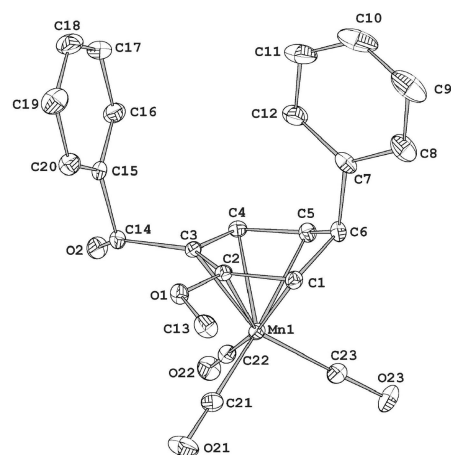
Figure 5. Molecular structure of complex 13a with thermal ellipsoids at the 30% probability level. Hydrogen atoms have been omitted for clarity.
