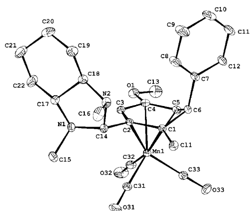
Figure 8. Molecular structure of complex ( R,R,6R,1pS )- 14 with thermal ellipsoids at the 30% probability level. Hydrogen atoms have been omitted for clarity.
