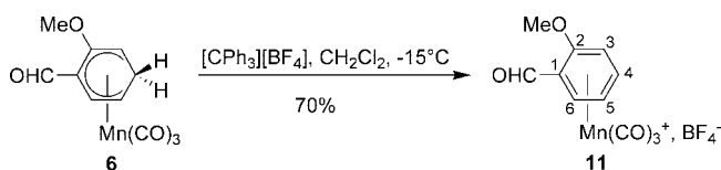
Scheme 1. Rearomatization of Complex (\eta^5\text{-3-Formyl-2-methoxycyclohexadienyl})\text{Mn}(\text{CO})_3 ( 6 )
