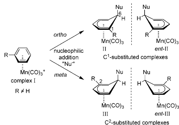
Figure 6. Chirality of ( \eta^5 -cyclohexadienyl)Mn(CO) 3 complexes.
