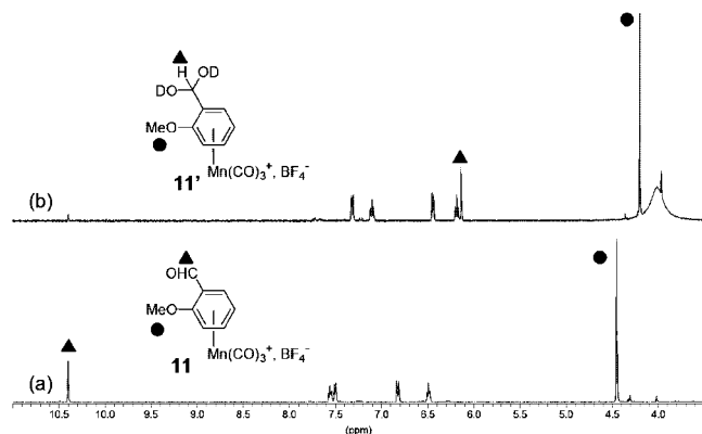
Figure 4. ^1\text{H} NMR spectra (400 MHz, acetone- d_6 ): (a) complex [(\eta^6\text{-1-formyl-2-methoxybenzene})\text{Mn}(\text{CO})_3][\text{BF}_4] 11 and (b) the corresponding gem -diol 11' after addition of \text{D}_2\text{O} .
