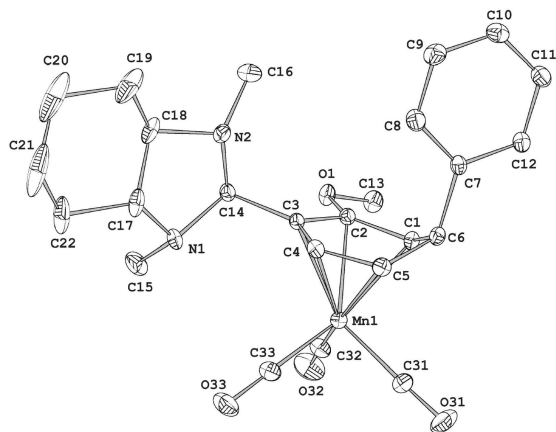
Figure 10. Molecular structure of complex (R,R,6S,2pR) - 15 15a with thermal ellipsoids at the 30% probability level. Hydrogen atoms have been omitted for clarity.
