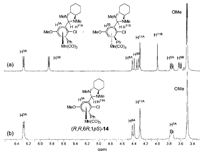
Figure 7. Selected sections of 1 H NMR spectra (200 MHz, CDCl 3 ): (a) crude mixture of diastereoisomers ( R,R,6R,1pS )- 14 and ( R,R,6S,1pR )- 14 ; (b) after chromatographic separation: ( R,R,6R,1pS )- 14 with ≥95% de.
