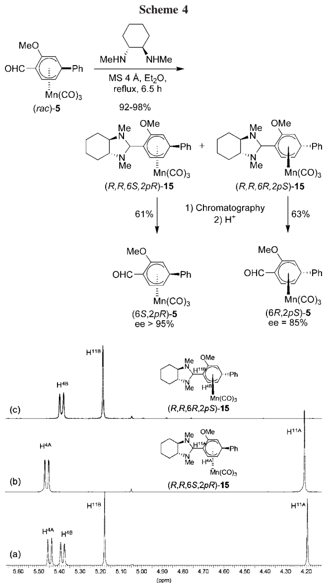
Figure 9. Selected sections of 1 H NMR spectra (400 MHz, CDCl 3 ): (a) crude mixture of diastereoisomers ( R,R,6S,2pR )- 15 and ( R,R,6R,2pS )- 15 ; after chromatographic separation, (b) ( R,R,6S,2pR )- 15 with ≥95% de and (c) ( R,R,6R,2pS )- 15 with ≥95% de.
