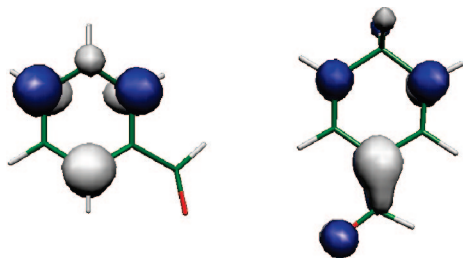
Figure 3. Highest occupied molecular orbitals for 10a (left) and 10b (right). Isodensity equal to 0.7.
