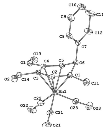
Figure 1. Molecular structure of complex 7b with thermal ellipsoids at the 30% probability level. Hydrogen atoms have been omitted for clarity.
