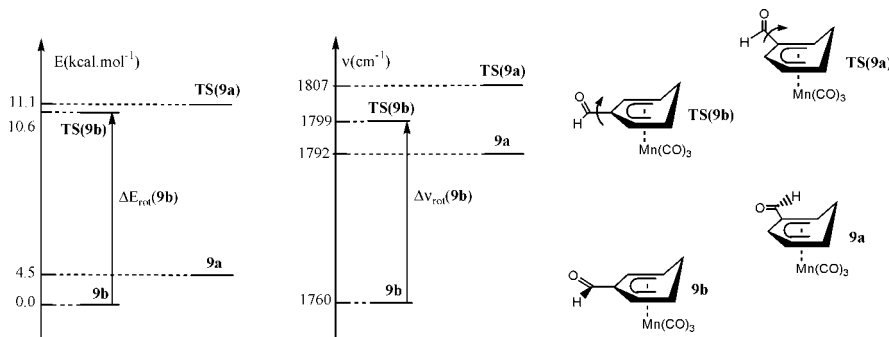
Figure 2. Computed \nu_{\text{CHO}} vibrational frequencies and energies (relative to the most stable structure) for the lowest energy conformers and for the lowest transition states of structures 9a and 9b .
