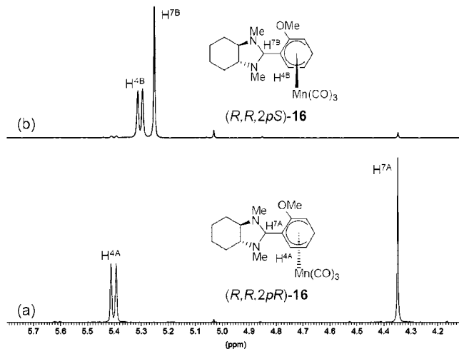
Figure 11. Selected sections of ^1H NMR spectra (400 MHz, CDCl_3 ): after chromatographic separation of the diastereoisomeric mixture (a) (R,R,2pR) - 16 ( \geq 95\% de) and (b) (R,R,2pS) - 16 (de = 92%).
