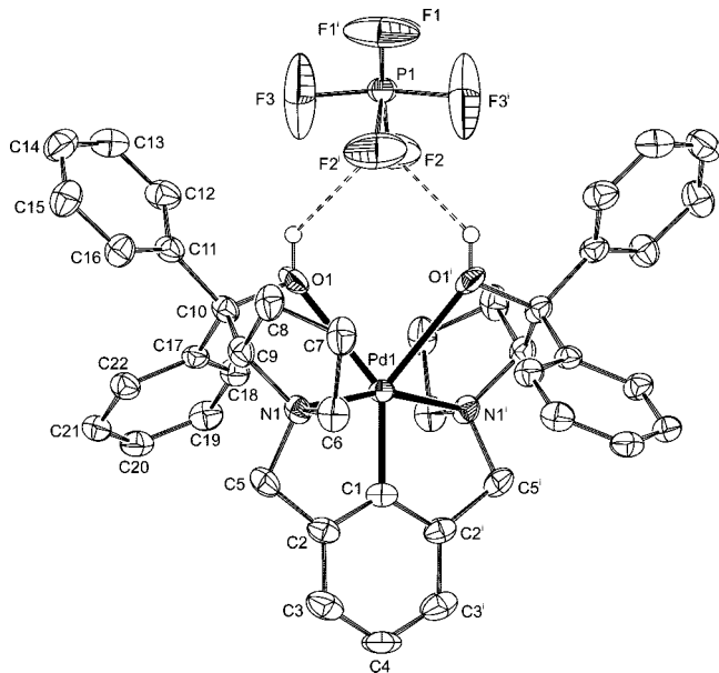
Figure 3. Displacement ellipsoid plot (50% probability) of complex [4]PF 6 with depicted intermolecular hydrogen bonds. Remaining hydrogen atoms are omitted for clarity. Symmetry operation i: y, x, −z.
