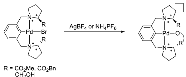
Scheme 1. Structures of Neutral and Cationic Pyrrolidine NCN-Pincer Complexes
