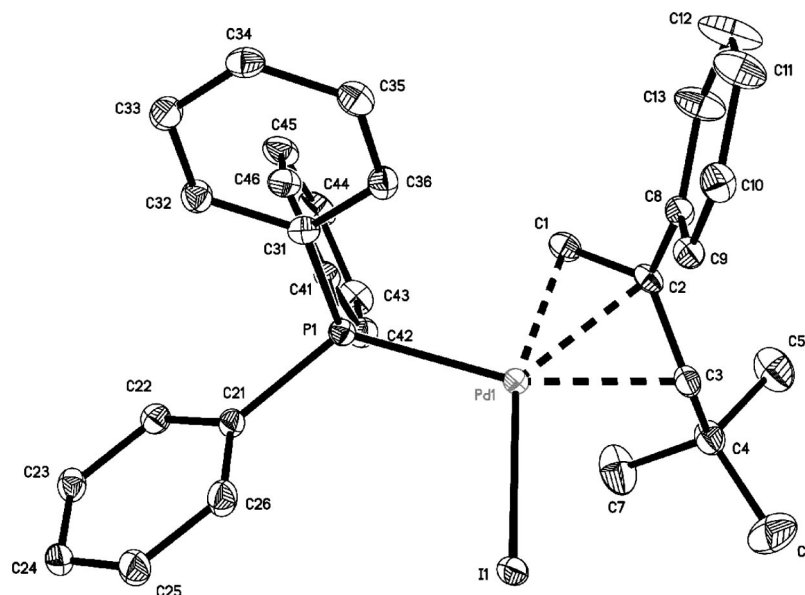
Figure 2. X-ray structure of compound trans -5 with thermal ellipsoids shown at the 40% probability level.
