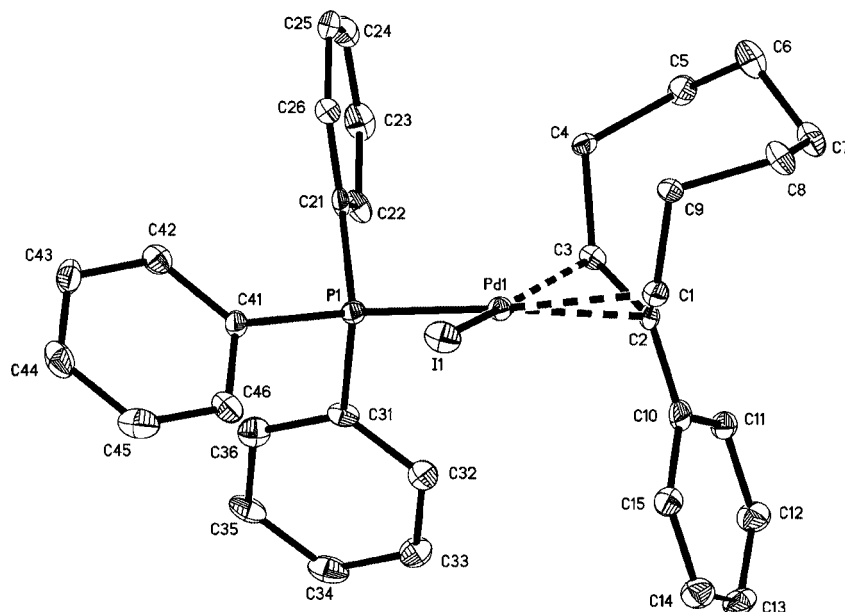
Figure 1. X-ray structure of compound 3 with thermal ellipsoids shown at the 40% probability level.
