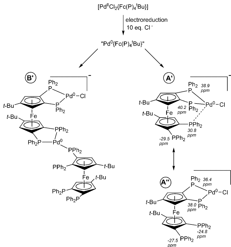
Scheme 4. Formation of Stabilized Zerovalent Palladium Species A'/A'' or B' in the Presence of 10 equiv of [n\text{-Bu}_4\text{N}][\text{Cl}] Salt
