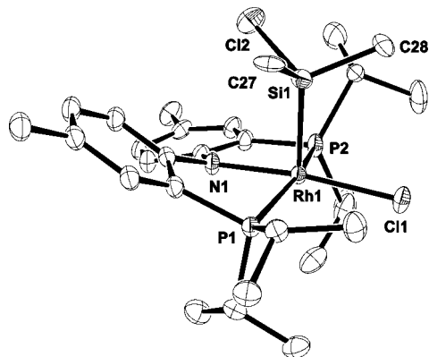
Figure 1. ORTEP 20 drawing (50% probability ellipsoids) of 7 showing selected atom labeling. Hydrogen atoms are omitted for clarity. Selected bond distances (Å) and angles (deg) follow: Rh1–Si1, 2.2777(9); Rh1–P1, 2.3249(8); Rh1–P2, 2.3256(8); Rh1–N1, 2.027(2); Rh1–Cl1, 2.3511(7); Si1–Rh1–P1, 96.46(3); Si1–Rh1–P2, 97.43(3); P1–Rh1–P2, 159.42(3); Si1–Rh1–N1, 91.56(8); P1–Rh1–N1, 80.38(7); P2–Rh1–N1, 84.13(7); Si1–Rh1–Cl1, 96.24(3); P1–Rh1–Cl1, 99.42(3); P2–Rh1–Cl1, 94.09(3); N1–Rh1–Cl1, 172.17(8).
