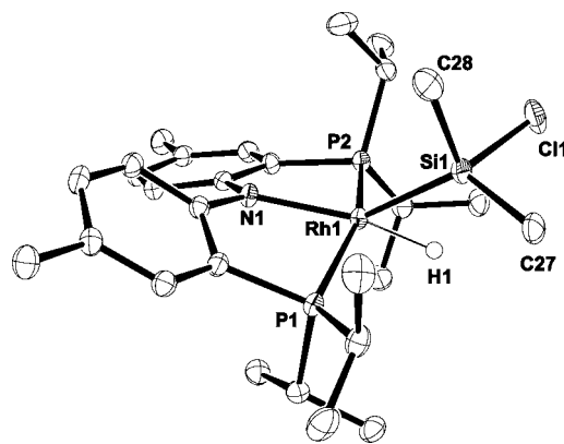
Figure 2. ORTEP 20 drawing (50% probability ellipsoids) of 15 showing selected atom labeling. Hydrogen atoms (except Rh–H) and the rotational disorder of the Me 2 SiCl group are omitted for clarity. Rotational disorder of the SiClMe 2 group is not shown. Selected bond distances (Å) and angles (deg) follow: Rh1–P1, 2.3081(4); Rh1–P2, 2.3056(4); Rh1–N1, 2.0642(13); Rh1–Si1, 2.2600(5); Rh1–H1, 1.50(2); Si1–H1, 1.93(2); P1–Rh1–P2, 156.195(16); P1–Rh1–N1, 80.62(4); P2–Rh1–N1, 82.58(4); P1–Rh1–Si1, 100.928(17); P2–Rh1–Si1, 102.866(17); N1–Rh1–Si1, 136.83(4); P1–Rh1–H1, 97.3(8); P2–Rh1–H1, 94.8(8); N1–Rh1–H1, 165.7(8).
