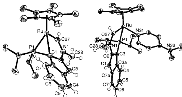
Figure 1. ORTEP diagrams for 3 (left) and 4·DMAP (right), shown with 50% displacement ellipsoids and with the atomic numbering scheme depicted; only one of the two crystallographically independent molecules of 3 is presented, and selected H-atoms have been omitted for clarity (DMAP = 4-dimethylaminopyridine).
