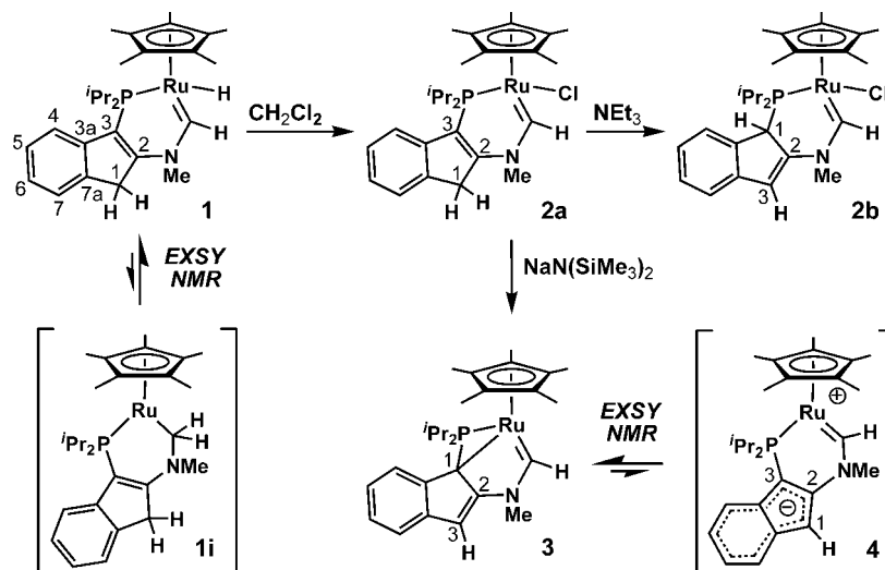
Scheme 1. Synthesis of 3 and the Reversible Formation of 4 (the Atomic Numbering Scheme Is Provided for Representative Complexes)
