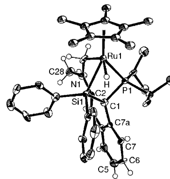
Figure 2. ORTEP diagram for 8 , shown with 50% displacement ellipsoids and with the atomic numbering scheme depicted; selected H-atoms have been omitted for clarity.
