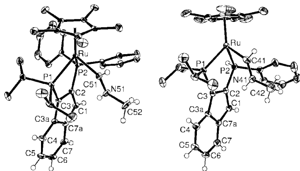
Figure 4. ORTEP diagrams for 12 (C 6 H 6 ) 2.5 (left) and 13 (right) shown with 50% displacement ellipsoids and with the atomic numbering scheme depicted; selected H-atoms and the benzene solvates have been omitted for clarity.
