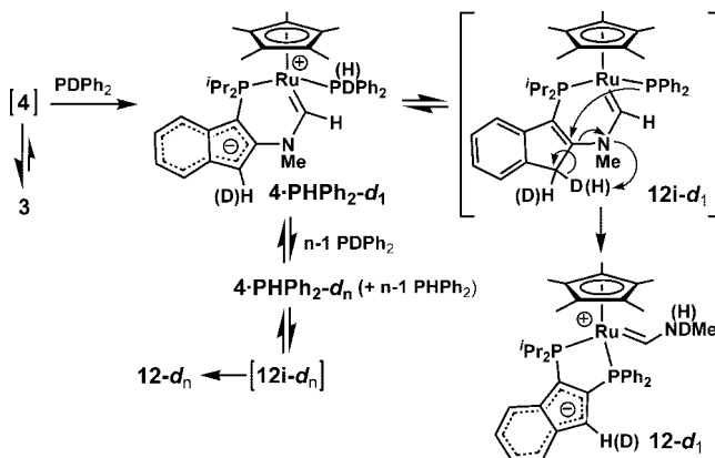
Scheme 7. Possible Mechanism for the Conversion of 4 ·PPh 2 to 12 on the Basis of a Deuterium Labeling Study
