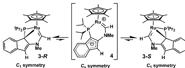
Scheme 2. Proposed Interconversion of Enantiomeric Forms of 3 via the \text{C}_s -Symmetric Intermediate 4 a
