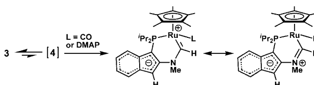
Scheme 3. Preparation of 4·L and an Important Resonance Contributor ( 4·L' ) for This Class of Complexes a
