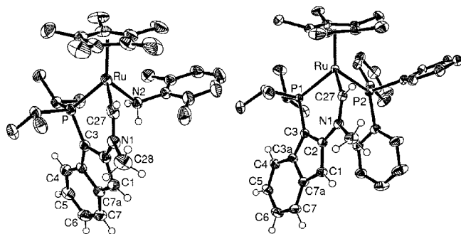
Figure 3. ORTEP diagrams for 4 \cdot \text{NC}_8\text{H}_{11}(2.5\text{NC}_8\text{H}_{11}) (left) and 4 \cdot \text{PPh}_3(\text{C}_6\text{H}_6) (right), shown with 50% displacement ellipsoids and with the atomic numbering scheme depicted; selected H-atoms, as well as the benzene and 2,6-dimethylaniline ( \text{NC}_8\text{H}_{11} ) solvates, have been omitted for clarity.
