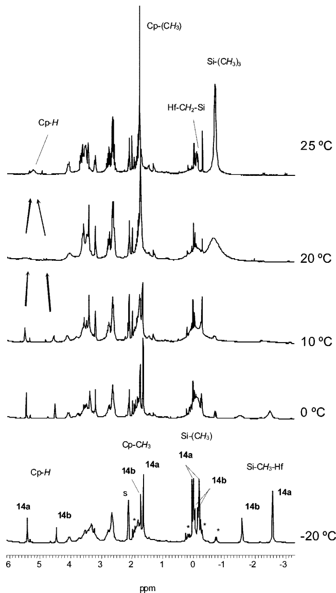
Figure 4. ^1\text{H} NMR spectrum (toluene- d_8 /1,2-difluorobenzene) of the cationic hafnium species obtained by the reaction of 14 with \text{CPh}_3[\text{B}(\text{C}_6\text{F}_5)_4] ( \text{Hf}:\text{B} = 1:1.1 ) at differing temperatures. Asterisks mark the \text{Hf}-\text{CHH}-\text{Si} peaks of both major ( 14a ) and minor ( 14b ) isomers.
