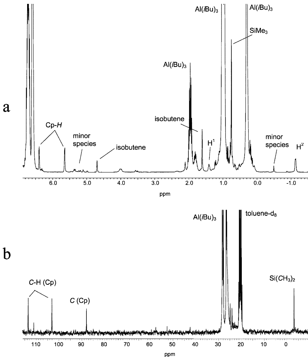
Figure 1. (a) ^1\text{H} and (b) ^{13}\text{C} NMR spectra of 9 obtained by the reaction of (\text{SBI})\text{HfCl}_2 ( 1 ) with \text{AlBu}_3/\text{CPh}_3[\text{B}(\text{C}_6\text{F}_5)_4] ( \text{Hf}:\text{Al}:\text{B} = 1:50:1.1 ; toluene- d_8 /1,2-difluorobenzene, 20^\circ\text{C} ).
