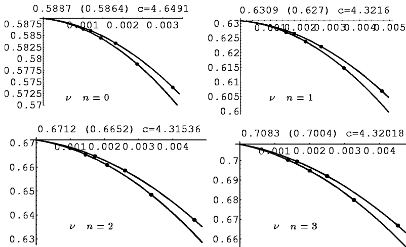
FIG. 2. Strong-coupling values for the critical exponent \nu^{-1} obtained from expansion (4) via formula (14), for increasing orders N=2, 3, \dots, 7 of the approximation. The exponents are plotted against the variable x_N = e^{-cN^{1-\omega}} and should for large n lie on a straight line. Here at finite N , even and odd approximants may be connected by slightly curved parabolas whose common intersection determines the critical exponents for N = \infty . More details on the determination of the constant c are given in the text. The numbers on top give the extrapolated critical exponents and, in parentheses, the highest approximants, to illustrate the extrapolation distance.
