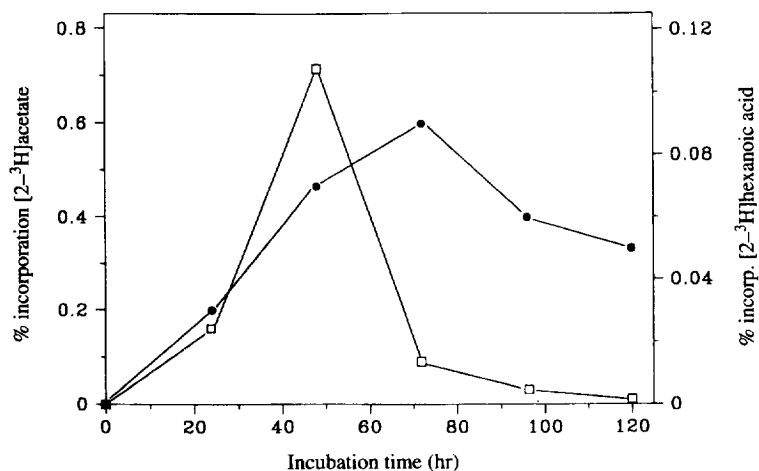
Fig. 1. Incorporation of ^3\text{H} into primin upon incubation of P. obconica leaves with □, [2-^3\text{H}] acetate and ●, [2-^3\text{H}] hexanoic acid (SD \pm 15\% ).
