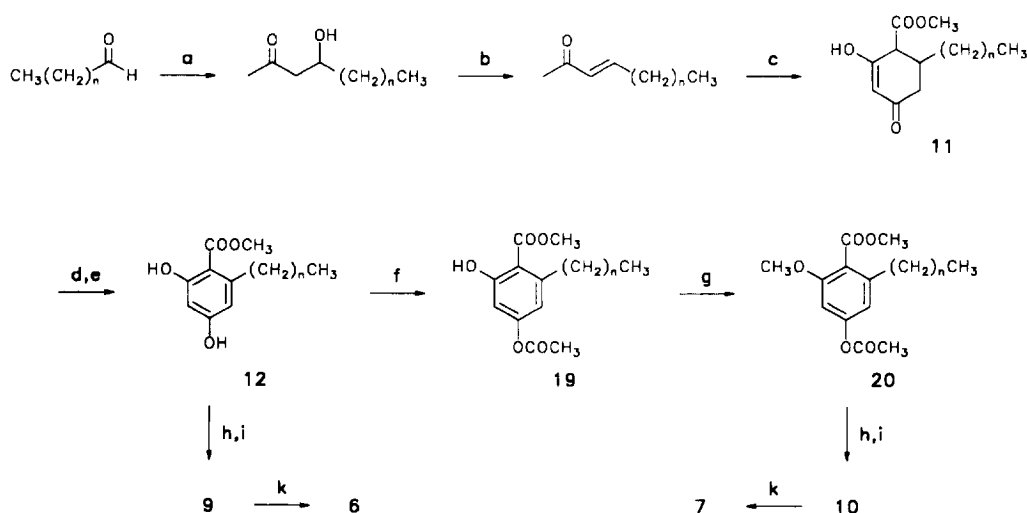
Scheme 2. Preparation of intermediates of primin biosynthesis ( n = 4 ) and their homologues ( n = 3, 5 ). Reagents: (a) \text{CH}_3(\text{CH}_2)_n\text{CHO} , NaOH. (b) TosOH. (c) \text{CH}_2(\text{COOCH}_3)_2 , NaOMe–MeOH. (d) \text{Br}_2 –DMF, 0^\circ . (e) \Delta ( 70 – 80^\circ ), 24 hr. (f) \text{Ac}_2\text{O} –pyridine, 0^\circ . (g) \text{CH}_3\text{I} – \text{K}_2\text{CO}_3 , acetone. (h) NaOH–MeOH. (i) HCl. (k) MeOH– \text{H}_2\text{O} , \Delta .
