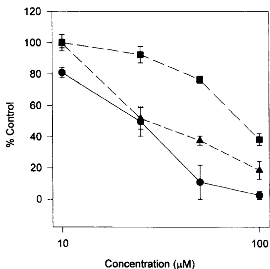
Fig. 4. Germination inhibition index of wheat as a percentage of control for (+)-ABA ( 1 , ●), (+)-C-1'-O-methyl ABA ( 4 , ■) and (-)-C-1'-O-methyl ABA ( 5 , ▲). Error bars represent the standard error of three replicates.
