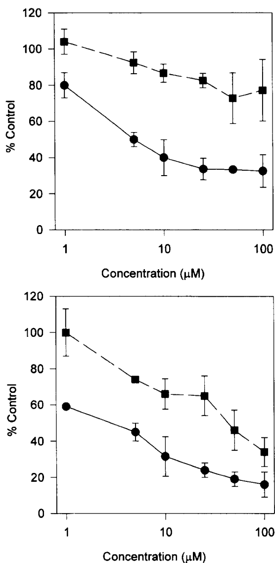
Fig. 2. Effect on transpiration rate of wheat seedlings of (+)-ABA ( 1 , ●) and (+)-C-1'-O-methyl ABA ( 4 , ■). At 3 hr, upper graph; at 8 hr, lower graph. Error bars represent the standard deviation of three replicates.
