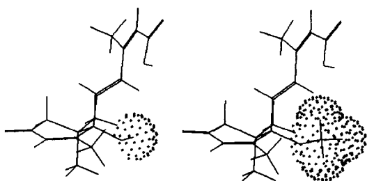
Fig. 1. Comparison of the van der Waals' radius of the hydrogen on the C-1'-hydroxyl group of ABA and the methyl group on the C-1'-O-methyl group of C-1'-O-methyl ABA. Generated in SYBYL ® software by TRIPOS Inc.
