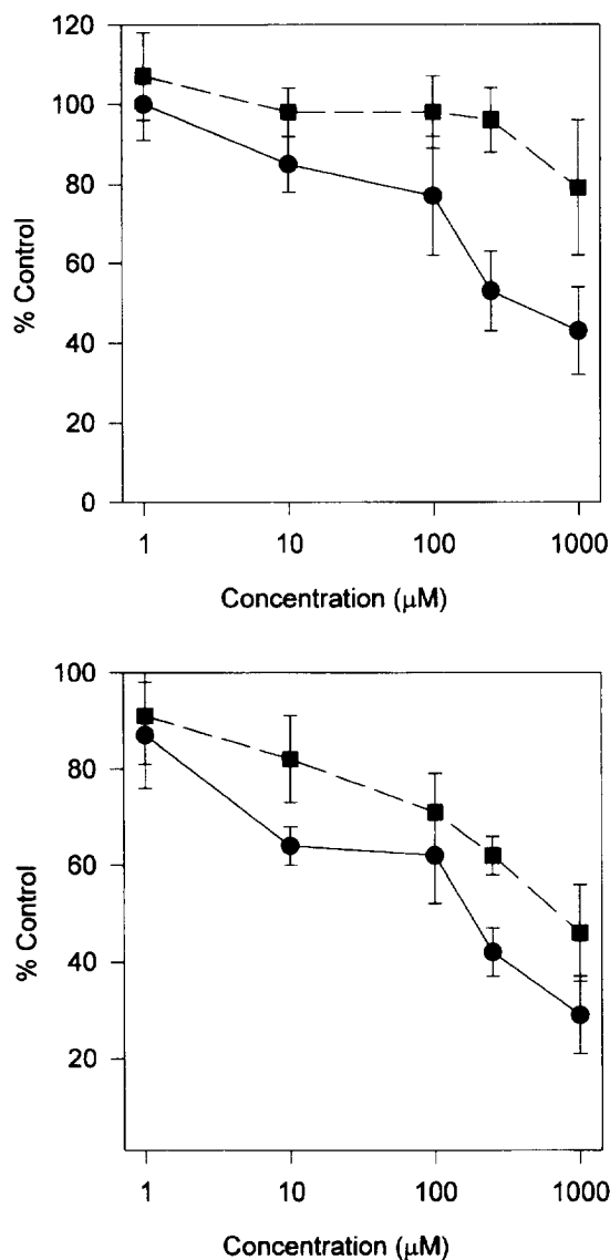
Fig. 3. Effect on transpiration rate of wheat seedlings of (–)-ABA ( 2 , ●) and (–)-C-1'-O-methyl ABA ( 5 , ■). At 3 hr, upper graph; at 8 hr, lower graph. Error bars represent the standard deviation of three replicates.
