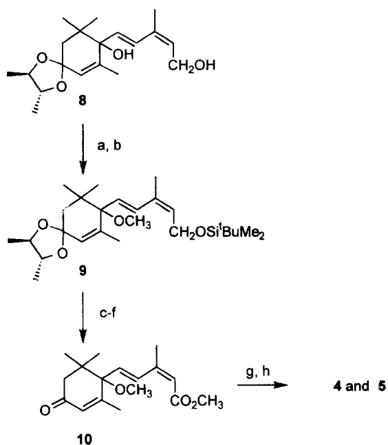
Scheme 1. Outline of synthesis of 4 and 5 . a: Tert -butyldimethylsilylchloride, imidazole; b: (i) methyllithium, (ii) methyl iodide; c: tetrabutylammonium fluoride; d: MnO 2 ; e: MnO 2 , NaCN, acetic acid, methanol; f: 10% HCl; g: HPLC resolution; h: porcine liver esterase.
