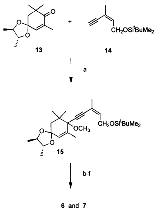
Scheme 2. Outline of synthesis of 6 and 7 . a: (i) n -Butyllithium, (ii) methyl iodide; b: tetrabutylammonium fluoride; c: MnO 2 ; d: MnO 2 , NaCN, acetic acid, methanol; e: 10% HCl; f: HPLC resolution.
