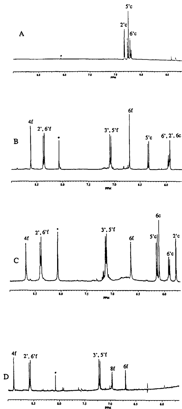
Fig. 3. 1 H NMR spectra of catechin (A), 4a (B), 4b (C) and flavylum ion 2 (D) (400 MHz, CD 3 OD/DCl, 27°). The signals of the catechin and flavylum ring B protons of 4a and 4b are strongly diamagnetically shifted with respect to the corresponding signals of 2 and catechin. ●, Formic acid (from HPLC eluents).
