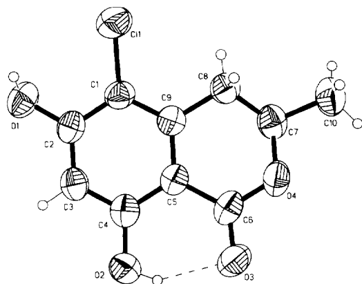
Fig. 2. The molecule of 5-chloro-6-hydroxymellein ( 2 ) in the crystal.
