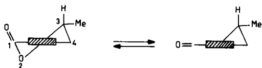
Fig. 4. Standard projection from the aromatic into the heterocyclic ring of (3 R )-(-)- 1c , (-)- 2 , (+)- 3 and (-)- 4 (half-chair and boat conformation, left and right, respectively).
