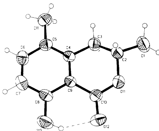
Fig. 1. The molecule of 5-methylmellein ( 1b ) in the crystal.
