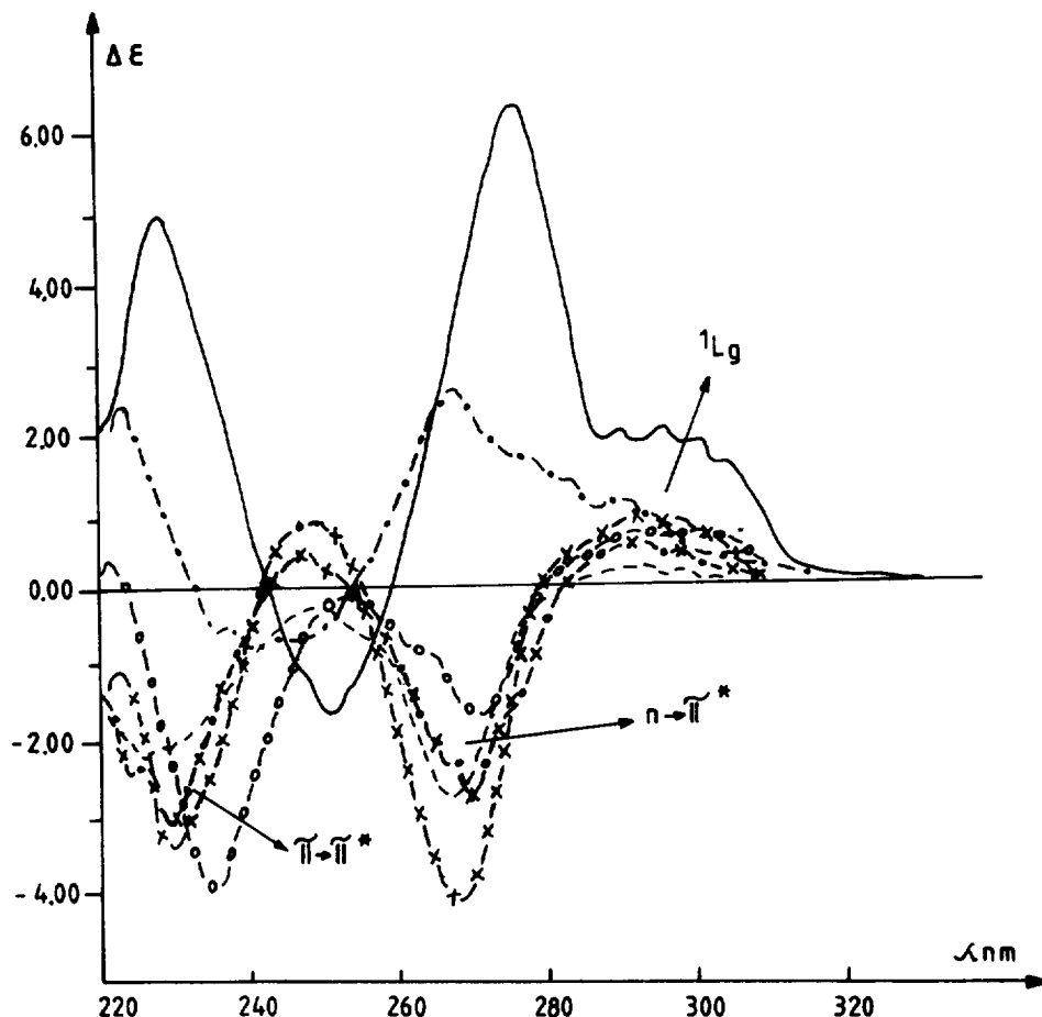
Fig. 3. CD curves of compounds (—)- 1c , (---)- 2c and (· · ·)- 8 in ethanol (—●—, —○—, —○—) and in n -hexane (—·—, —·—, —●—), respectively.
