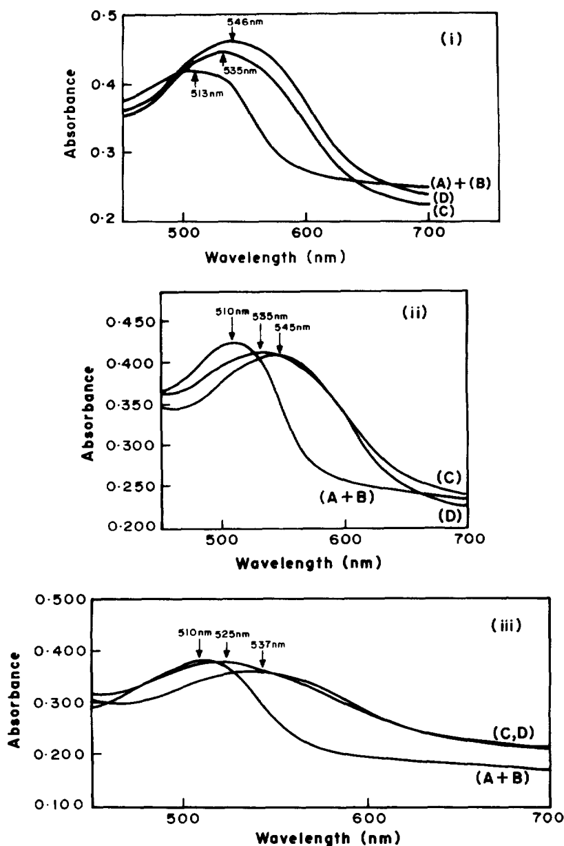
Fig. 2. Absorption spectra of cyanidin derivative from (i) Oryza sativa , (ii) Zea mays , and (iii) garden roses: (A) 6 \mu M cyanidin derivative; (B) 6 \mu M cyanidin derivative and 15 \mu l of 10 mM AsA; (C) 6 \mu M of cyanidin derivative and 10 \mu l of 5% of \text{AlCl}_3 ; and (D) 6 \mu M cyanidin derivative, 15 \mu l of 10 mM AsA and 10 \mu l of 5% of \text{AlCl}_3 in 50 mM NaOAc buffer pH 4. The spectra were recorded after incubating the mixtures for 1 hr at room temperature.
