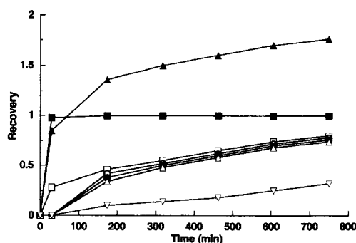
Fig. 1. Hydrolysis of angiotensin I by carboxypeptidase W. See text for experimental details. ■, Leu; ▲, His; □, Phe; ○, Pro; ●, Ile; △, Tyr; ▽, Val.
