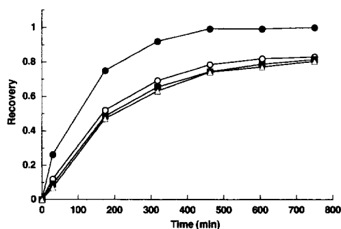
Fig. 2. Hydrolysis of eledoisin-related peptide by carboxypeptidase W. See text for experimental details. ●, Met-NH 2 ; ○, Leu; □, Gly; △, Ile.
