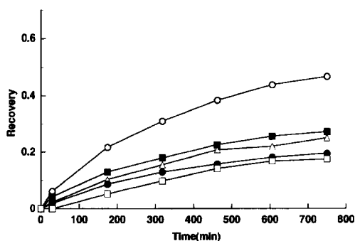
Fig. 3. Hydrolysis of [D-Ala 2 , Met 5 ]-enkephalinamide by carboxypeptidase W. See text for experimental details. ○, Met-NH 2 + Met; □, Met; △, NH 3 ; ●, Met-NH 2 ; ▫, Phe.
