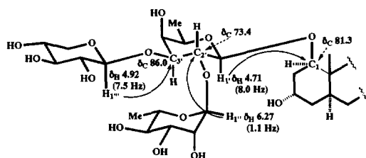
Fig. 1. HMBC correlations of the saccharide portion of 1 .
