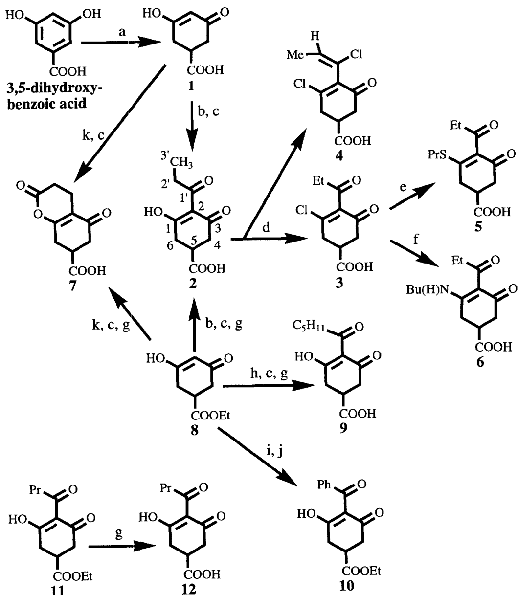
Scheme 1. Structures and synthesis of acylcyclohexanedione-related inhibitors. a : Raney Ni-H 2 -NaOH; b : propionyl chloride-Et 3 N-CH 2 Cl 2 ; c : DMAP-CH 2 Cl 2 ; d : oxalyl chloride-DMF-CH 2 Cl 2 ; e : nPrSH-Et 3 N-THF; f : nBuNH 2 -Et 3 N-THF; g : 1 M NaOH; h : hexanoyl chloride-Et 3 N-CH 2 Cl 2 ; i : benzoyl chloride-Et 3 N-CH 2 Cl 2 ; j : acetone cyanohydrin-CH 3 CN; k : acryloyl chloride-Et 3 N-CH 2 Cl 2 .
