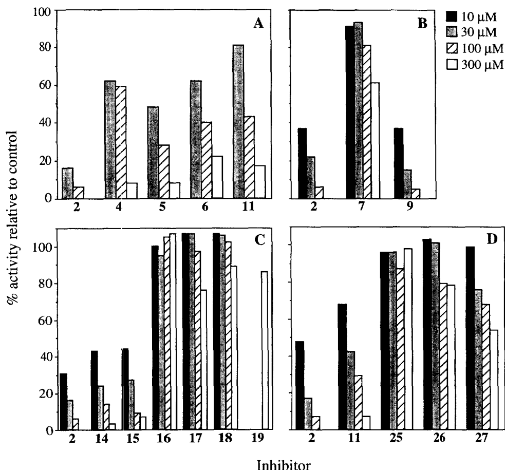
Fig. 2. Comparison of several 1- and acyl-substituted acylcyclohexanediones (A and B, respectively), substituted pyridines (C) and some other commercially-available compounds (D) with prohexadione (2) and LAB 198999 (11) as inhibitors of a partially-purified 3\beta -hydroxylase from C. maxima endosperm.
