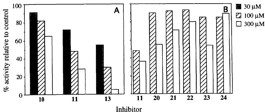
Fig. 3. Comparison of several 1-substituted acylcyclohexanedione ethyl esters (A) and hydroxy- and methoxybenzoic acids (B) with LAB 198999 ( 11 ) as inhibitors of a partially-purified 3 \beta -hydroxylase from C. maxima endosperm.
