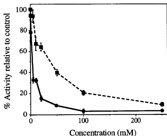
Fig. 1. Comparison of Prohexadione ( 2 , solid line) and its chloro-analogue ( 3 , dashed line) as inhibitors of partially-purified 3 \beta -hydroxylase from C. maxima endosperm.
