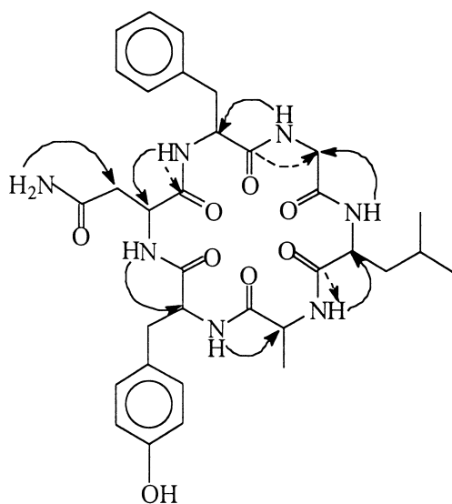
Fig. 1. Selected ROESY (→) and COLOC (---→) for dianthin A(1) in pyridine- d 5 .
