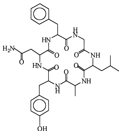
dianthin A(1)
