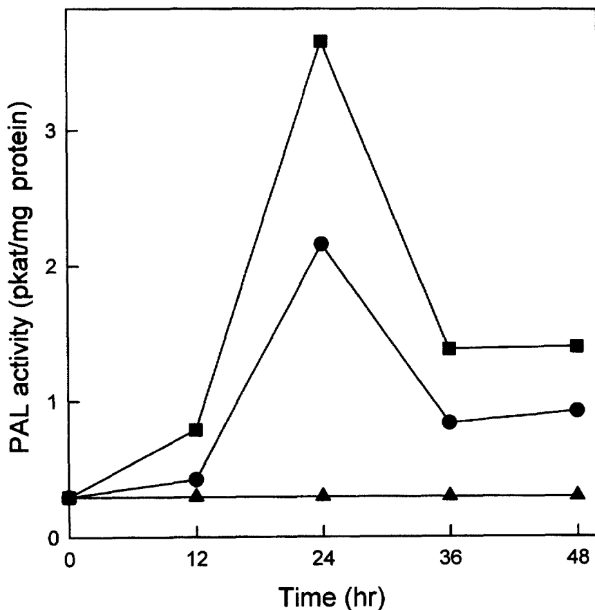
Fig. 1. Effect of excision on PAL activity of tomato leaves. The tomato seedlings were grown under continuous light for three weeks. Three grams (fr. wt) of tomato leaves were excised and were either incubated in dark (●) or in continuous light (■). The control leaves (▲) were obtained from intact seedlings. At the time intervals indicated, leaves were homogenised and the homogenate was processed till protamine sulphate step. PAL activity and protein were determined after dialysing the supernatant obtained after protamine sulphate precipitation.
