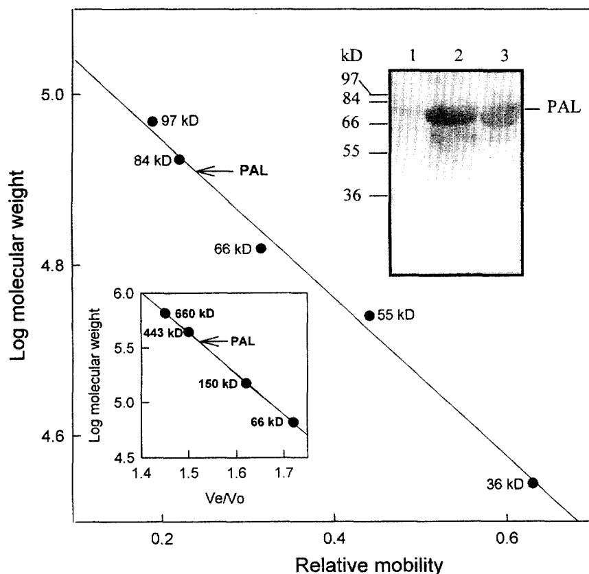
Fig. 3. Determination of M_r of PAL. The PAL subunit M_r was estimated by SDS-PAGE, using a calibration curve obtained for relative mobilities of markers run on a 12% acrylamide gel (see, materials and methods). The upper inset shows the Western blot of PAL after SDS-PAGE; Lane 1, crude-extract; Lane 2, pooled fraction from phenyl-Sepharose and Lane 3, pooled fraction from gel-filtration. The M_r of standard proteins are indicated on the left margin of the inset. The lower inset shows calibration curve used to determine the native M_r of PAL by gel-filtration chromatography on a Sepharose CL-6B column.
