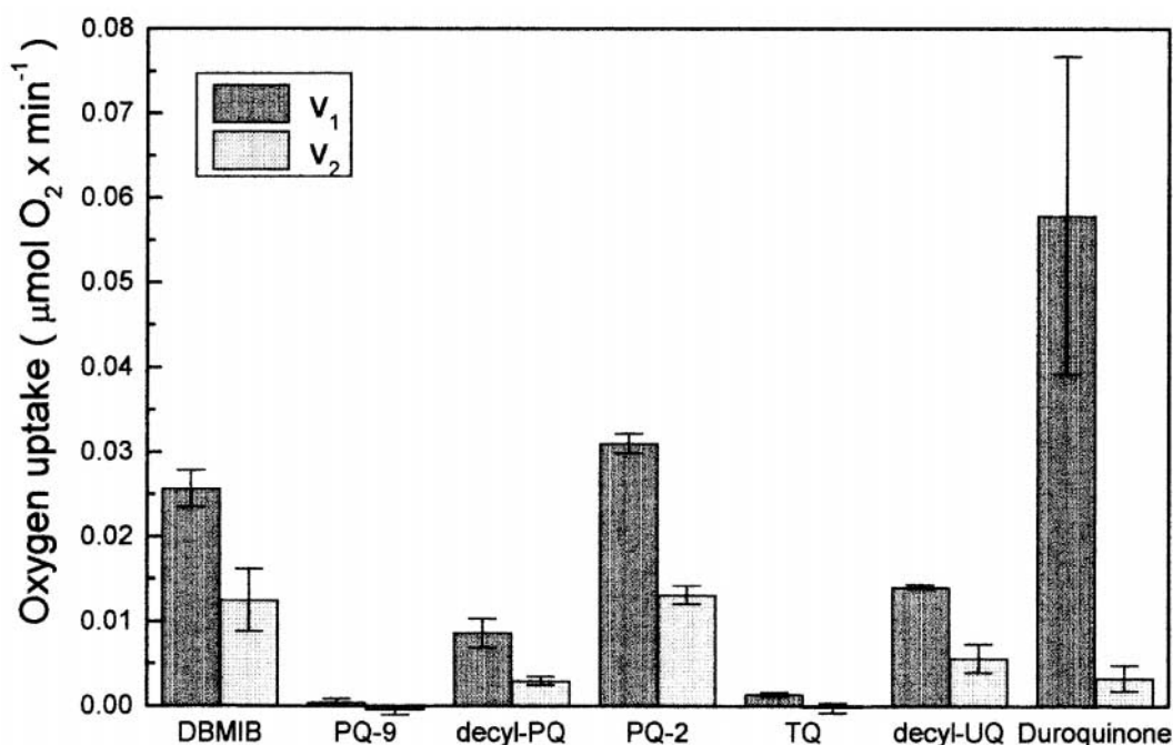
Fig. 2. NADPH (1 mM) initiated oxygen uptake ( V_1 , V_2 values) by the reaction mixture containing also 0.6 \mu\text{M} FNR and 20 \mu\text{M} quinone as indicated. Other details as in Fig. 1. DBMIB, dibromothymoquinone; PQ-9, plastoquinone-9; decyl-PQ, decyl-plastoquinone; PQ-2, plastoquinone-2; \alpha -TQ, \alpha -tocoquinone; decyl-UQ, decyl-ubiquinone.
