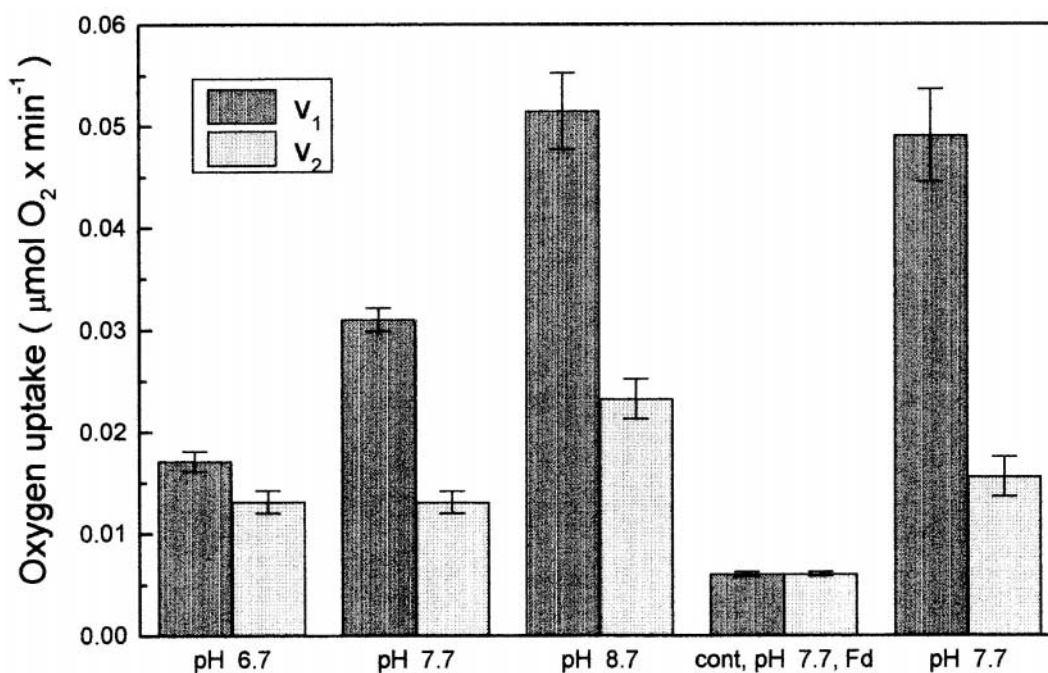
Fig. 3. Effects of pH (6.7, 7.7, 8.7) or ferredoxin, Fd (0.6 \mu\text{M} , as indicated) on the NADPH (1 mM) initiated oxygen uptake in the reaction mixture containing 0.6 \mu\text{M} FNR and 20 \mu\text{M} PQ-2. For the composition of the basic reaction mixture and other details see Fig. 1.
