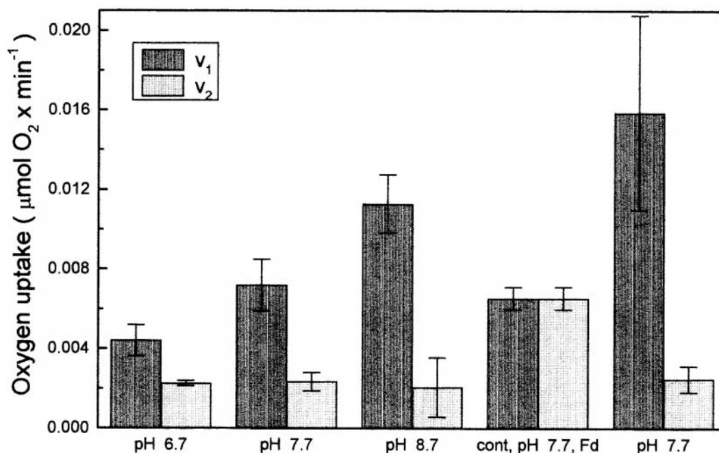
Fig. 4. The effects of pH (6.7, 7.7, 8.7) or Fd (0.6 \mu M, as indicated) on the NADPH (1 mM) initiated oxygen uptake by the reaction mixture containing 0.6 \mu M FNR and 20 \mu M decyl-PQ. For composition of the basic reaction mixture and other details see Figs. 1 and 2.
