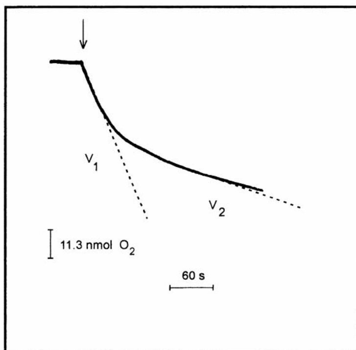
Fig. 1. Typical record of NADPH (1 mM)-initiated oxygen uptake by the buffered (pH 7.7, 40 mM Tris-HCl) reaction mixture (1 cm 3 ) containing 1 mM Na 2 EDTA, 1 mM MgCl 2 , 0.6 \mu M FNR and 20 \mu M duroquinone (or other quinones). V_1 , rate of oxygen uptake during the 1st minute of measurement; V_2 , rate of oxygen uptake between 2nd and 3rd minutes of measurement.
