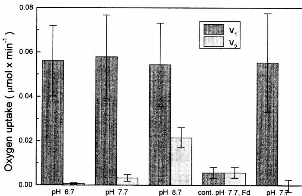
Fig. 5. Effect of pH (6.7, 7.7, 8.7) or Fd (0.6 \mu M, as indicated) on the NADPH (1 mM) initiated oxygen uptake by the reaction mixture containing 0.6 \mu M FNR and 20 \mu M duroquinone. For composition of the basic reaction mixture and other details see Figs. 1 and 2.
