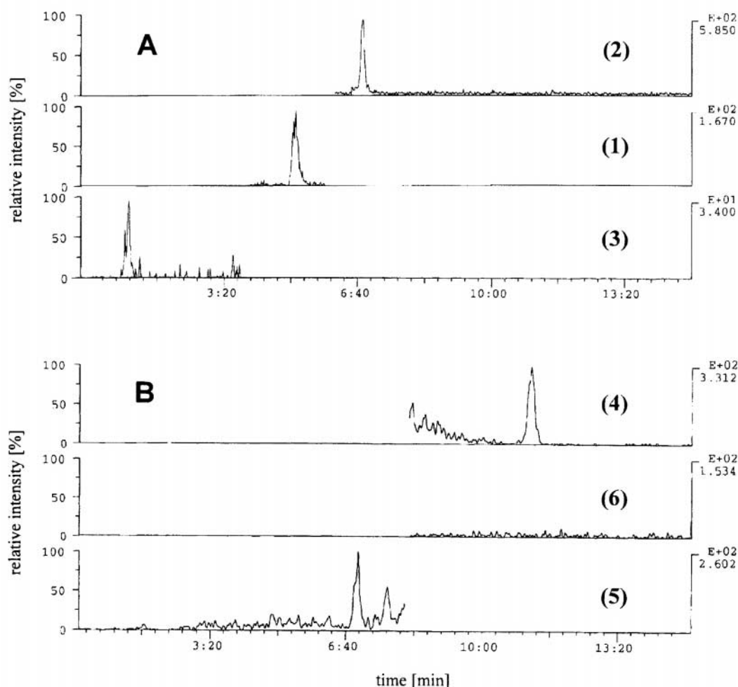
Fig. 2. Time-dependent SRM experiments for compounds 1–6 in strawberry leaf extract. Chromatogram A shows the product ion traces of group 1: 1–3 (SRM 1). The characteristic ion pairs are as follows: m/z 207.0/127.1 (3), 187.1/96.1 (1), 201.1/97.2 (2). Compound 3 ( RR_t 2.5 min) was not detectable in this sample. Chromatogram B shows the product ion traces of group 2: 4–6 (SRM 3). The characteristic ion pairs are as follows: m/z 303.3/97.2 (4), 273.3/97.2 (5), 233.2/96.2 (6). Compound 6 ( RR_t 10.2 min) was not detectable in this sample (ESI, negative mode, RP-18; gradient: 10 mM \text{NH}_4\text{Ac} in \text{H}_2\text{O} –10 mM \text{NH}_4\text{Ac} in 90% MeOH).
