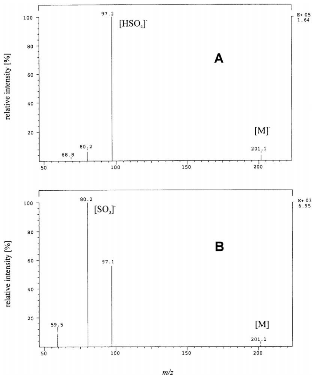
Fig. 1. Product ion mass spectra of 2 obtained by collision induced dissociation (CID) with different offset voltages (presursor ion: m/z 201.1 [M]^- ): (A) offset voltage 21 eV; (B) offset voltage 57 eV.
