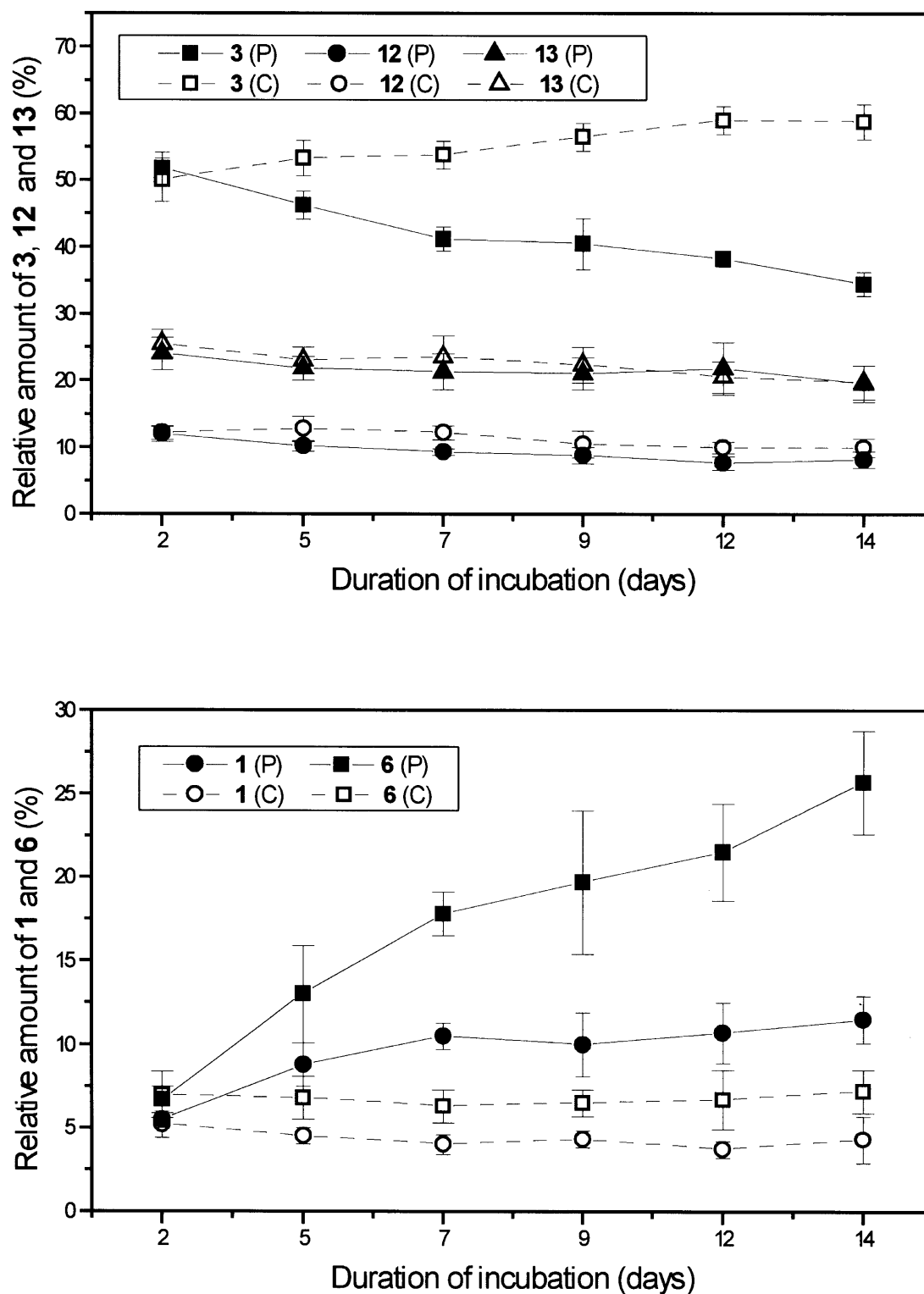
Fig. 1. Iridal composition (%) of an I. pseudacorus cell culture upon incubation with 3-amino-1,2,4-triazole. Top: spiroiridal 3 , 28-hydroxyspiroiridal 12 and 28-acetoxyspiroiridal 13 . Bottom: iridal 1 and 10-desoxyiridal 6 . Straight lines: probe and dashed lines: control.
