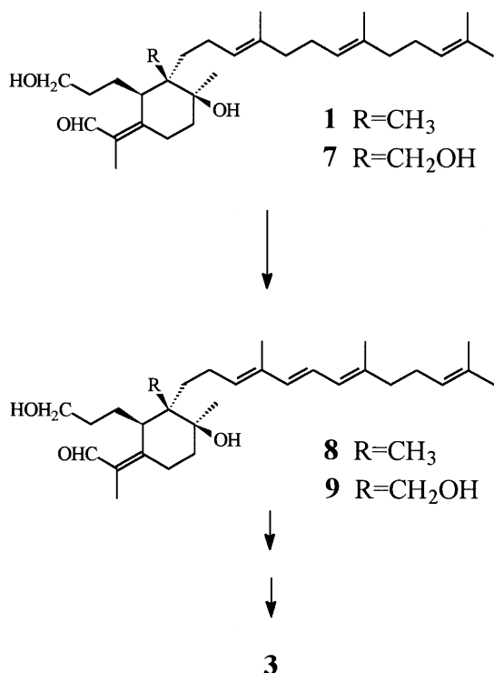
Scheme 2. Formation of the iridotrienes.
