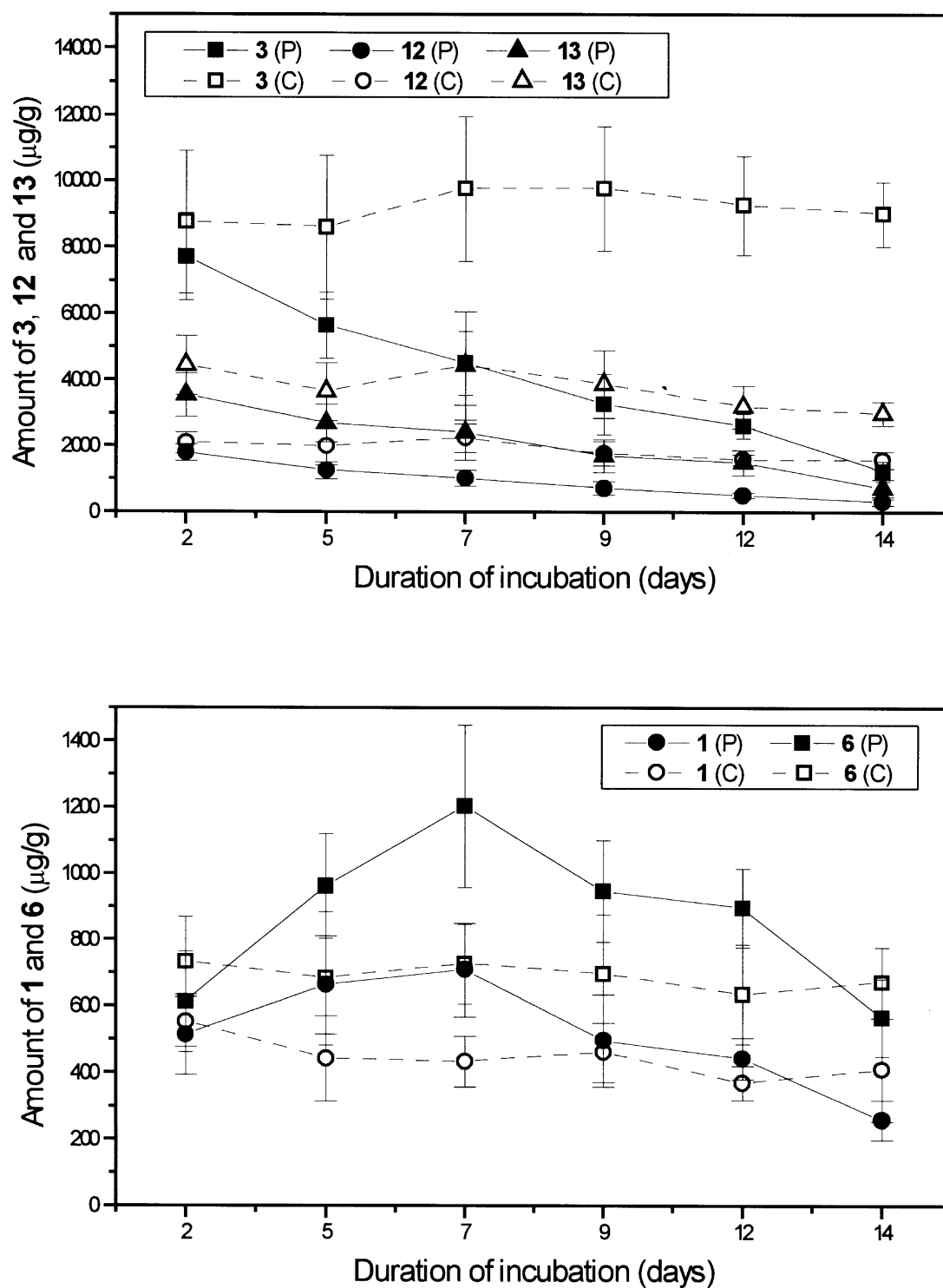
Fig. 3. Absolute amount of iridals (μg/g dry weight) in I. pseudacorus cells upon incubation with 3-amino-1,2,4-triazole. Top: spiroiridal 3, 28-hydroxyspiroiridal 12 and 28-acetoxyspiroiridal 13. Bottom: iridal 1 and 10-desoxyiridal 6. Straight lines: probe and dashed lines: control.
