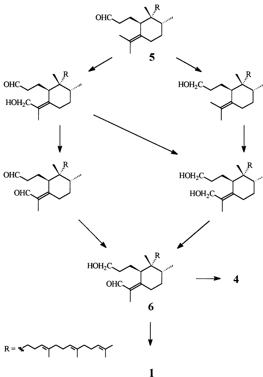
Scheme 1. Proposed biosynthesis of iridals and 10-desoxyiridals.
