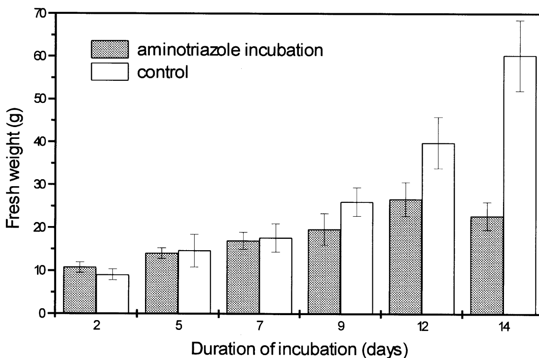
Fig. 2. Growth of an I. pseudacorus cell culture (fresh weight of cells) upon incubation with 3-amino-1,2,4-triazole.
