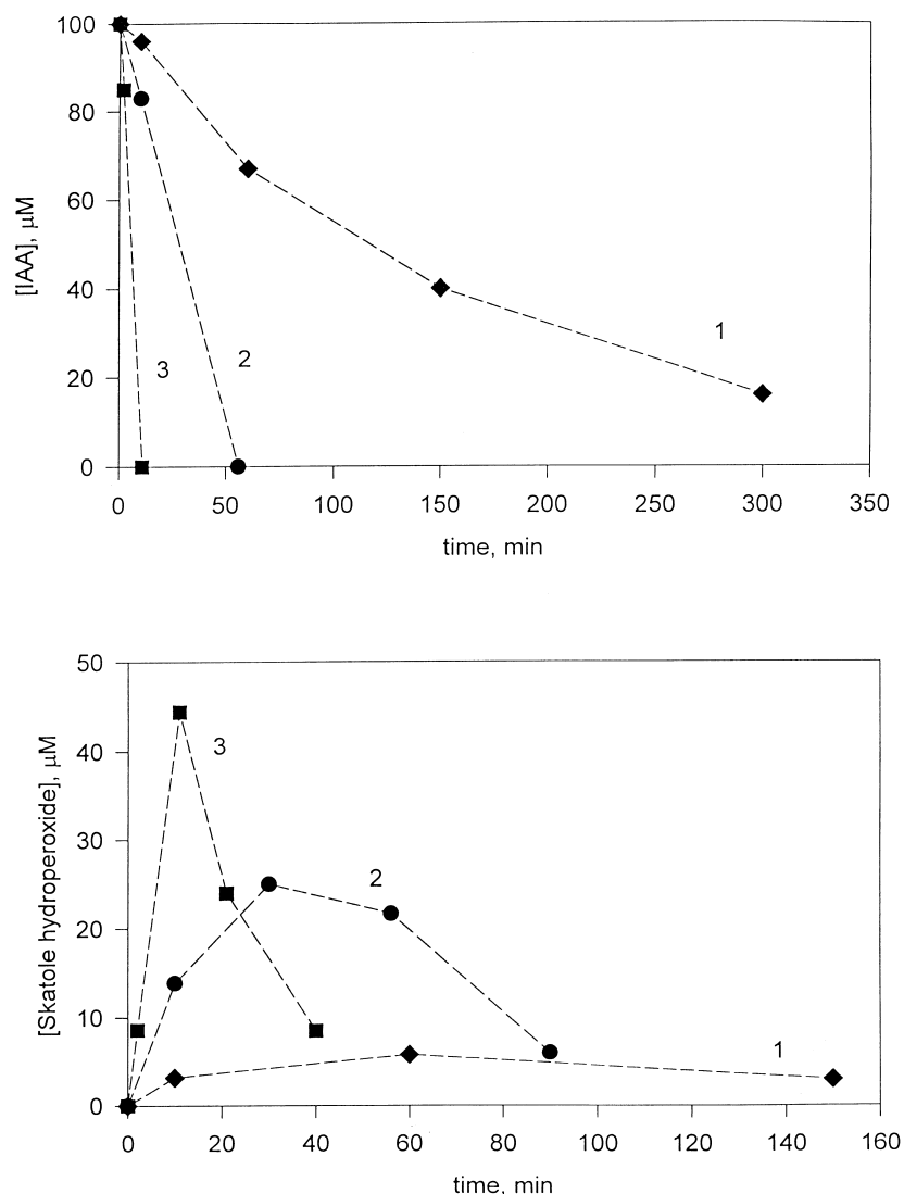
Fig. 4. The effect of PNP-C concentration on the kinetics of: (A) IAA degradation; (B) skatole hydroperoxide formation; (C) indole-3-aldehyde formation; (D) indole-3-methanol formation. All the reactions were in 0.1 M Na-acetate buffer, pH 5.0 with PNP-C concentrations of 1 , 0.07 \mu\text{M} ; 2 , 0.4 \mu\text{M} ; 3 , 1.4 \mu\text{M} .
