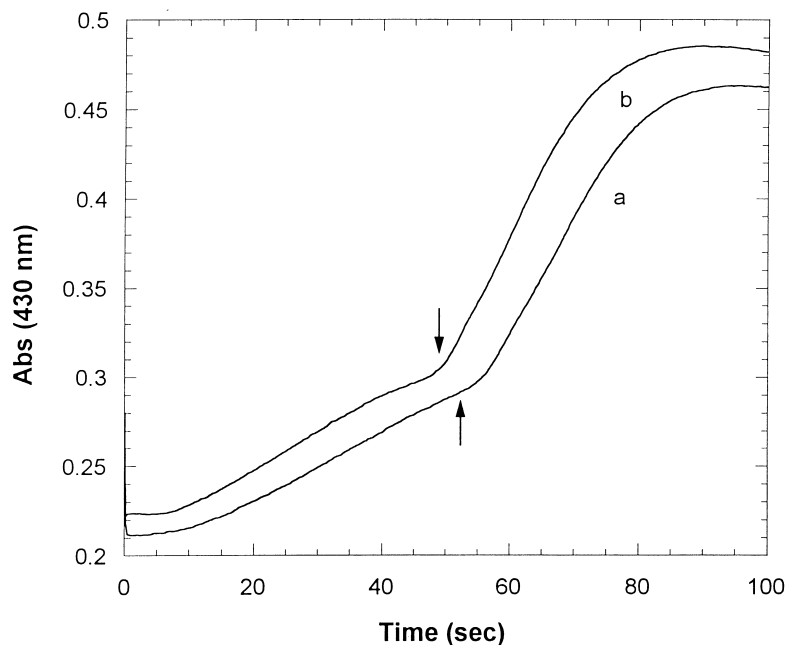
Fig. 3. The effect of superoxide dismutase (SOD) on the transient kinetics of IAA oxidation by molecular dioxygen catalysed by cationic peanut peroxidase (PNP-C) in 0.1 M Na-acetate buffer, pH 5.0, 22°. Traces recorded at 430 nm. (A) no additives; (B) 3 \mu M SOD. Reagent concentrations: 8 \mu M PNP-C, 5 mM IAA and 62.5 \mu M O 2 . The enzyme was shot against IAA-O 2 mixture, SOD was subsequently added to the IAA/O 2 solution. The arrows indicate the time at which ferrous enzyme begins to appear which corresponds to dioxygen exhaustion.
