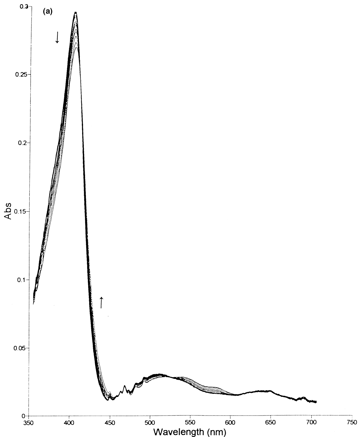
Fig. 2. Spectral changes occurring in the course of the reaction of 1 mM IAA with 4 \mu M peanut cationic peroxidase (PNP-C) in O_2 -containing buffer (62.5 \mu M). 0.1 M Na-acetate buffer, pH 5.0 22°. (A) 200 scans recorded in 100 s, and (B) 200 scans in 500 s, with every tenth scan shown. The arrows indicate the direction of change in absorbance with time.
