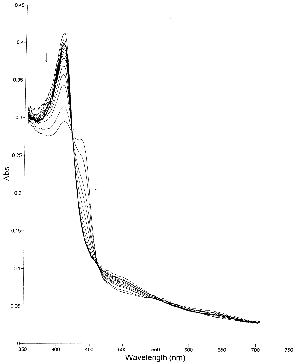
Fig. 1. Spectral changes occurring in the course of the reaction of 1 mM IAA with 4 \mu M peanut anionic peroxidase (PNP-A) in O_2 -containing buffer (62.5 \mu M), 0.1 M Na-acetate buffer, pH 5.0, 22°. (A) 200 scans recorded in 600 s, with every tenth spectrum shown. The arrows indicate the direction of change in absorbance with time.
