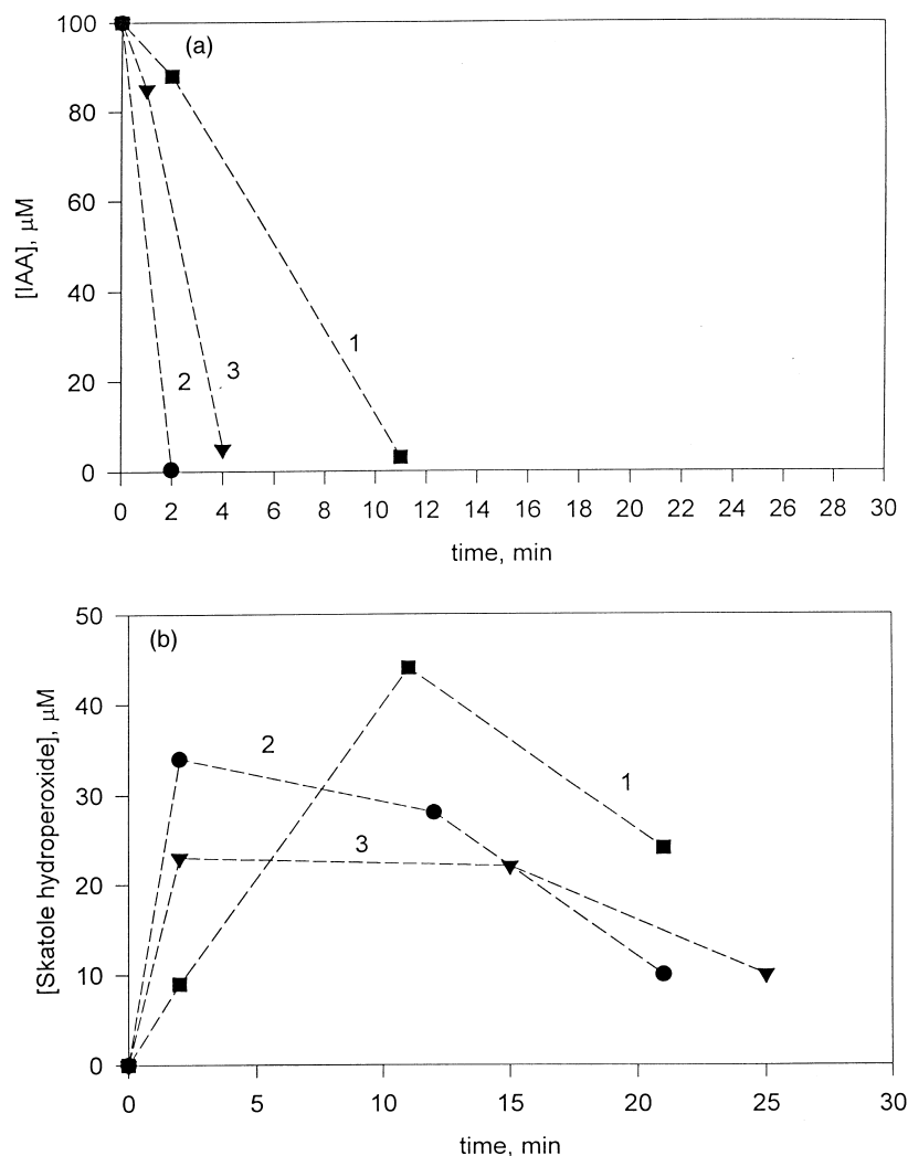
Fig. 5. Effect of superoxide dismutase (SOD, 0.3 \mu\text{M} ) and/or catalase (0.05 mg/ml) on the PNP-C (1.4 \mu\text{M} ) catalysed kinetics of: (A) IAA degradation; (B) skatole hydroperoxide formation; (C) indole-3-methanol formation; (D) indole-3-aldehyde formation. 1. No additives; 2, addition of SOD; 3, co-addition of catalase and SOD.
