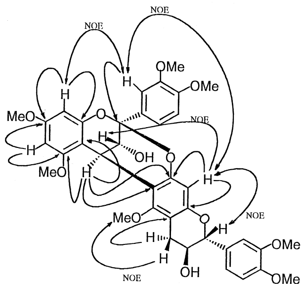
Fig. 1. NOE associations for determination of [2\rightarrow7, 4\rightarrow6] double linkage and COLOC experiments for determination of quaternary carbons. Arrows other than those labeled NOE correspond to COLOC correlations.
